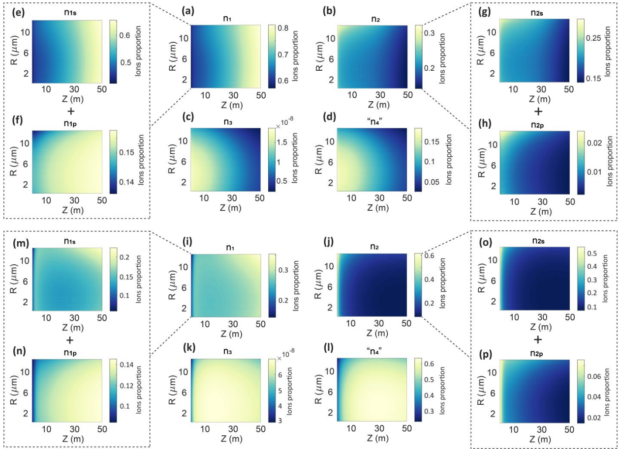
Figure 9. Distributions of erbium ions among energy levels on the cross-section (R) and along the Z-axis of the fiber at different pump powers. (a)-(d) and (i)-(l) are the ion distributions of level 1~level “4” at the pump power of 50 W and 2300 W, respectively. (e) and (f) are single-ion and paired-ion distributions on level 1 at the pump power of 50 W, respectively. (g) and (h) are single-ion and paired-ion distributions on level 2 at the pump power of 50 W, respectively. (m) and (n) are single-ion and paired-ion distributions on level 1 at the
