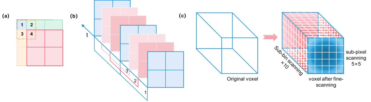
Fig 1 Schematic of the 3D sub-voxel scanning method. (a). An illustration of sub-pixel scanning using the SPAD array with 2 \times 2 pixels and an inter-pixel spacing of 1/2 FoV. (b). A scheme of sub-bin scanning in time domain with 3 steps. (c). One original voxel in the measurement matrix can be expanded to 5 \times 5 \times 10 sub-voxels after fine scanning.
