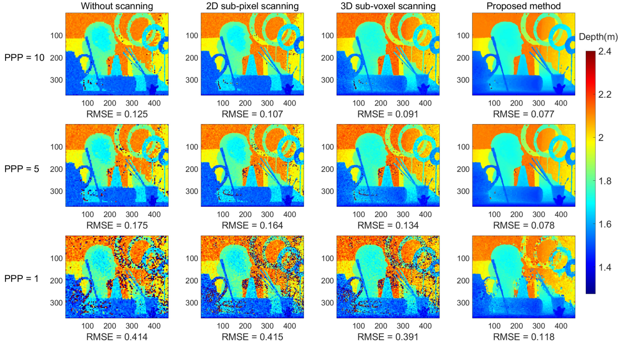
Fig 2 Numerical simulation of the proposed algorithm. The ground truth is a typical scene from the Middlebury dataset. In our simulation, the SBR is set to 0.2 and the average number of detected signal photons is set to 10, 5, and 1 PPP respectively. The first column shows the results without fine scanning. The second column shows the results with only 2D sub-pixel scanning and conventional pixel-wise ML processing. The third column shows the results with 3D sub-voxel scanning and pixel-wise ML processing. The last column shows the results with 3D sub-voxel scanning and our photon-efficient 3D deconvolutional algorithm. Quantitative results in terms of root mean square error (RMSE) are shown at the bottom of each figure. Clearly, our 3D sub-voxel method combined with the proposed algorithm has a smaller RMSE and superior performance to exhibit the details of the images.
