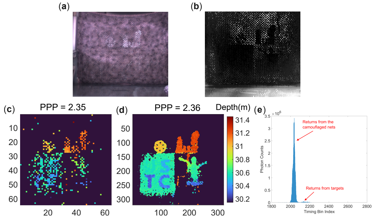
Fig 5 Experiment results of the static scenario behind the camouflage nets in daylight. The results of (a) visible-light camera, (b) MWIR camera, (c) single-photon LiDAR without fine scanning, (d) Single-photon LiDAR with 3D sub-voxel scanning, and (e) The timing histogram of the data in (d)
