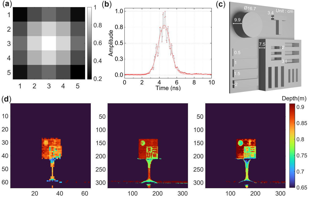
Fig 4 Calibration results of our imaging system. (a). The calibration result of the PSF_{2D} including 5 \times 5 pixels. (b). The calibration result of Box(t) * IRF(t) . The red line is the Gaussian fit of the raw data. (c). The 3D model of the resolution chart. (d). The results were captured by single-photon LiDAR without fine scanning, with 2D sub-pixel scanning, and with 3D sub-voxel scanning, separately.
