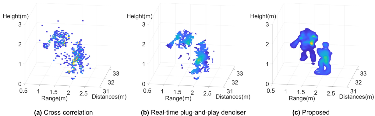
Fig 9 Comparison of 3D reconstruction methods for moving targets behind the camouflage nets. The data is the same as the first frame displayed in Fig. 8. Reconstruction results of (a) cross-correlation, (b) real-time plug-and-play denoiser, 15 and (c) the proposed method.
