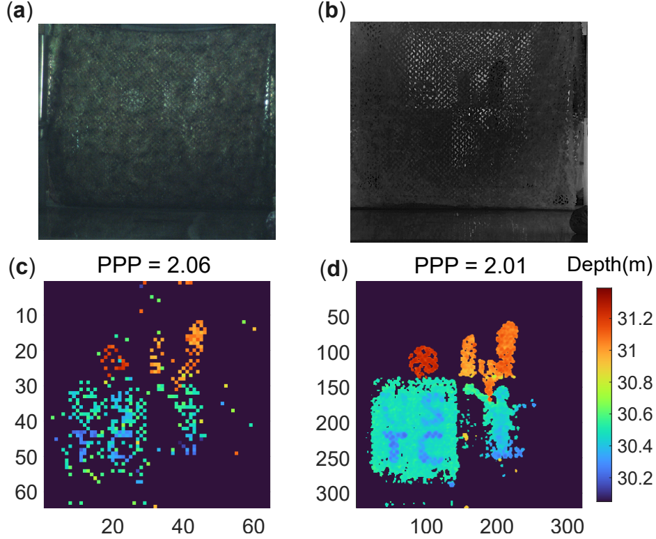
Fig 7 Experiment results of the static scenario behind the camouflage nets at night. The results of (a) visible-light camera, (b) MWIR camera, (c) single-photon LiDAR without fine scanning, and (d) Single-photon LiDAR with 3D sub-voxel scanning. (a) and (b) are applied with contrast enhancement for better visual effects.
