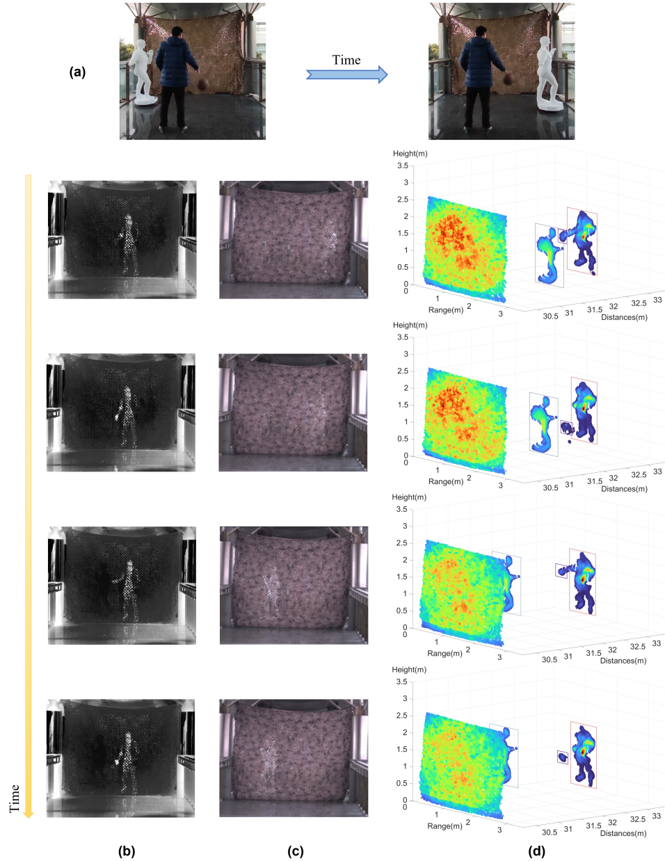
Fig 8 Experiment results of the moving scenario behind the camouflage nets. (a). The photographs of the scene behind the camouflage nets taken from backward. (b). The photographs were captured by MWIR camera. (c). The photographs were captured by a visible-light camera. (d). The reconstructed 3D profile of the multi-layer scenario. The movement of the mannequin and the basketball can be seen in the image sequences. The boxes of different colors indicate the segmented objects in our experiment.
