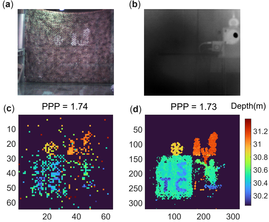
Fig 6 Experiment results of the static scenario behind the camouflage nets in daylight with a glass door. The results of (a) visible-light camera, (b) MWIR camera, (c) single-photon LiDAR without fine scanning, and (d) Single-photon LiDAR with 3D sub-voxel scanning. (a) and (b) are applied with contrast enhancement for better visual effects.
