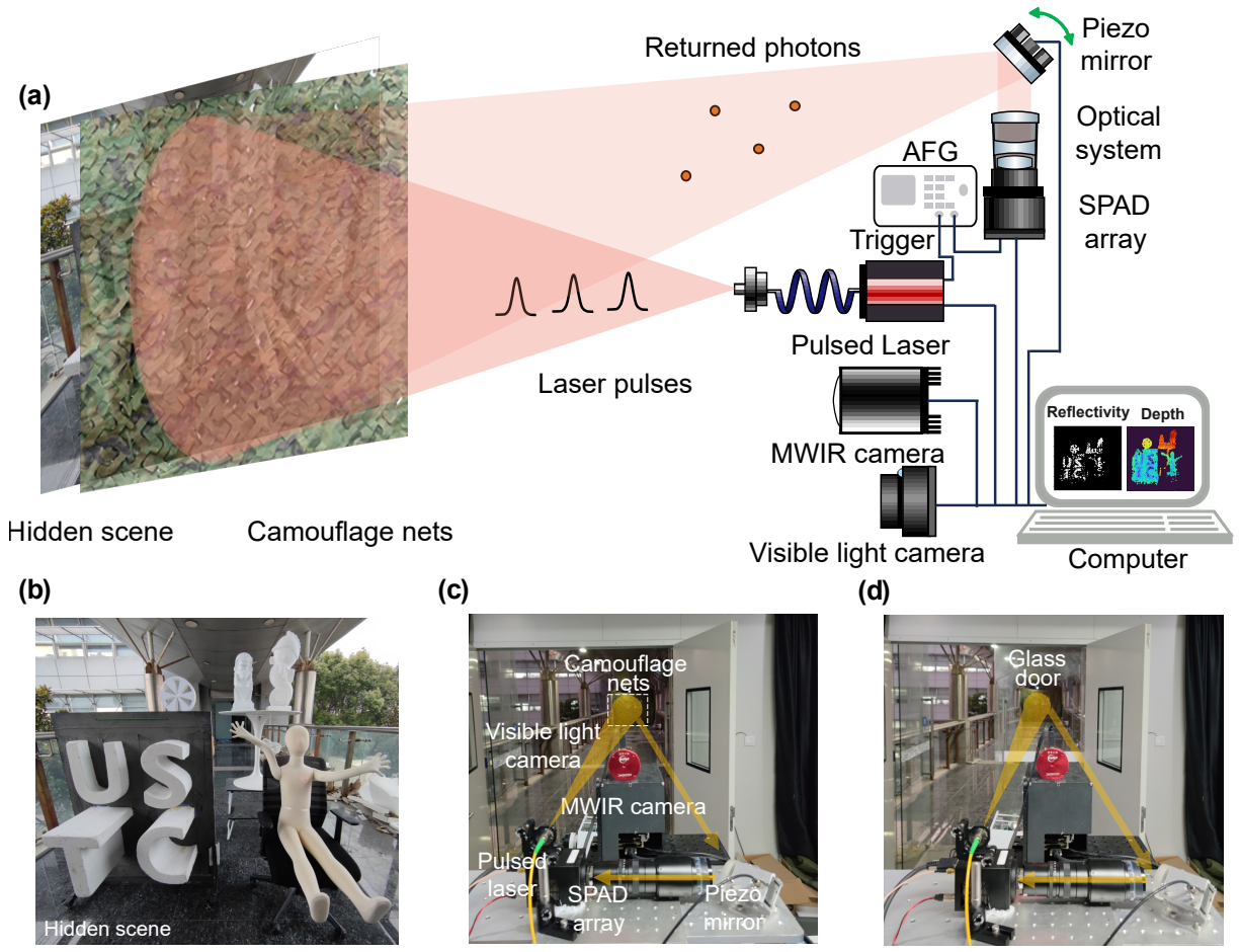
Fig 3 Schematic diagram of the experimental setup. (a). The schematic diagram of our experiment setup. The complex scenario is hidden behind a double-layer camouflage net, which is imaged by a visible-light camera, a MWIR camera, and our single-photon LiDAR system. (b). The photograph of the hidden scene. (c). The photograph of our experiment setup. (d). A photograph during the experiment with the glass door closed as an obstruction in the imaging path.
