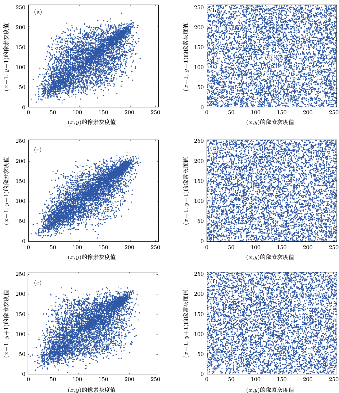
图 9 baboon 图像加密前后三个方向上的相关性分析图 (a), (b) 对角相邻; (c), (d) 水平相邻; (e), (f) 垂直相邻; Fig. 9. Correlation analysis chart in three directions before and after baboon image encryption: (a), (b) Diagonally adjacent; (c), (d) horizontally adjacent; (e), (f) vertically adjacent.
