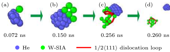
图 1 单晶 W 中氦团簇成核长大初期的位错环发射过程 Fig. 1. The punching-loop at the early stage of nucleation and growth of helium clusters in bulk W.
