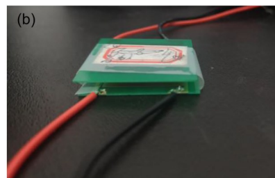
图 12 叠层氚基同位素电池的结构模型(a)及实物图(b) Fig.12 Structural model (a) and physical diagram (b) of stacked tritium-based nuclear battery
