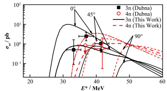
图3 DNS模型对 48 Ca+ 238 U反应生成Cn同位素的理论产生截面与实验值的比较 [26] Fig.3 Comparison of calculated DNS model results with experimental data in the production cross sections of Cn isotopes in the 48 Ca+ 238 U reaction [26]
