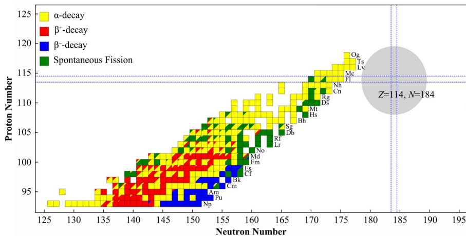
图1 截至到2022年底已知的317超重核素 Fig.1 The 317 transuranium nuclides that were known by the end of 2022
