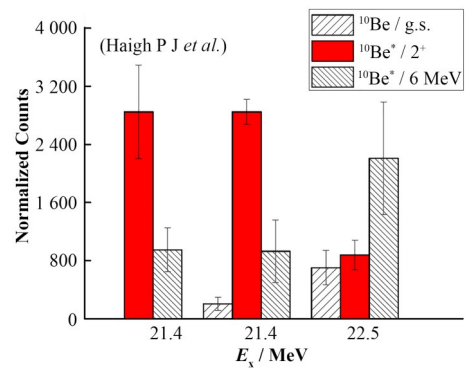
图7 ^{14}\text{C} 的21.4 MeV和22.5 MeV的共振态衰变到 ^{10}\text{Be} (不同量子态)+ \alpha 的相对分支比 [15] Fig.7 ^{14}\text{C} \rightarrow ^{10}\text{Be} + \alpha relative branching ratio for 21.4-MeV and 22.5-MeV resonances in ^{14}\text{C} with respect to three sets of final states in ^{10}\text{Be} obtained from the present measurement [15]
