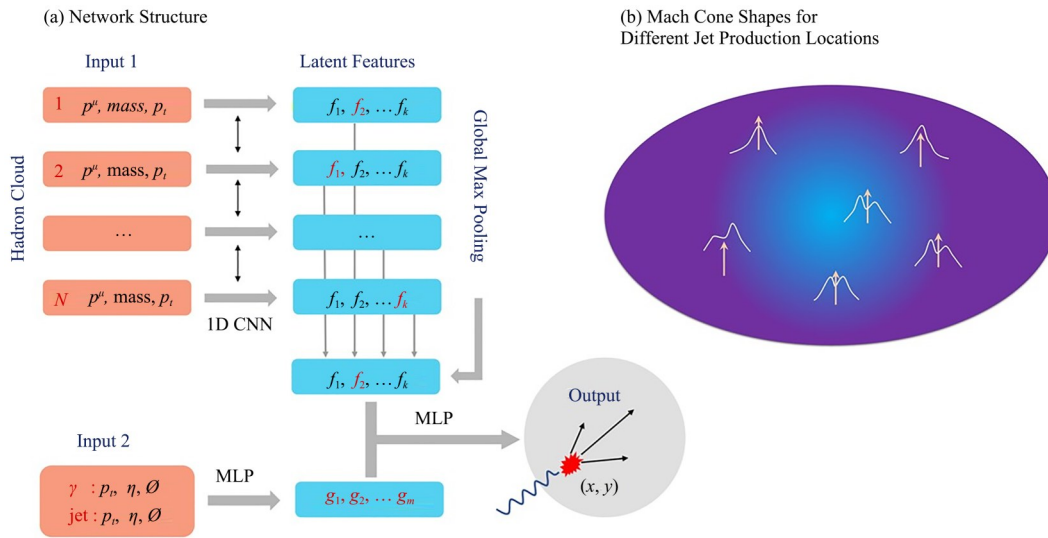
图 12 深度学习辅助的喷注层析技术,定位高能粒子的初始产生位置,帮助寻找核液滴中的马赫锥 [58] Fig.12 Deep learning assisted jet tomography used to locate the initial jet production positions and aid in searching the Mach cone in nuclear liquid [58]
