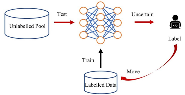
图 9 主动学习 (Active learning) 的流程图 [43] Fig.9 Flow chart illustrating active learning [43]
