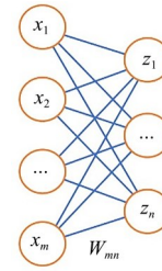
图4 单层人工神经网络对数据的变换等价于线性矩阵操作 z=xW+b ,再使用非线性激活函数将 z 的每个元素进行变换 Fig.4 A single layer artificial neural network transforms the input data by a linear matrix operation z=xW+b , in combination with a non-linear operation on each element of the output z using a non-linear activation function
