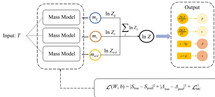
图8 使用深度神经网络构造3个温度依赖的质量函数,并且计算配分函数从而获得QCD的状态方程 [42] Fig.8 Framework of the deep neural network when constructing three temperature-dependent mass functions and calculating the QCD EoS using DNN learned masses [42]
