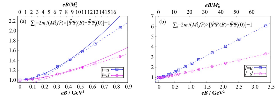
图4 零温下手征凝聚与磁场强度的变化关系 [21] (a) 弱场的情况,(b) 扩展到强场的情况 Fig.4 eB dependences of chiral condensate at eB < 0.9 \text{ GeV}^2 (a) and with eB up to 3.5 \text{ GeV}^2 (b) [21]
