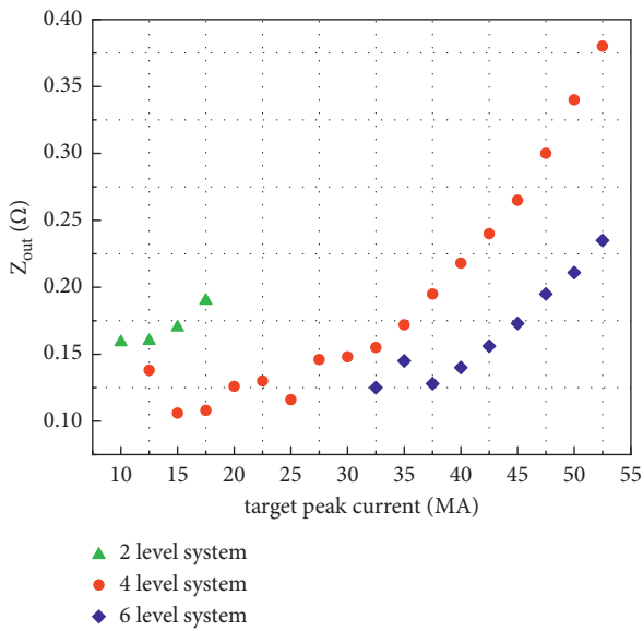
FIGURE 8: The output impedance of MRTL versus target peak load current with different transmission line systems.
