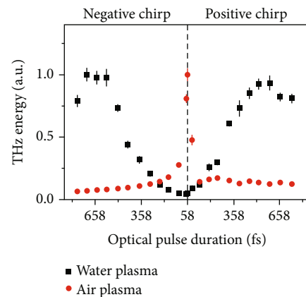
FIGURE 7: Normalized THz energy with different optical pulse durations [10]. THz signal generated by water plasma prefers an optical excitation with a longer pulse duration. However, the THz wave generation from air plasma is always in favor of the shortest pulse. The optical pulse energy is 0.4 mJ for both cases.
