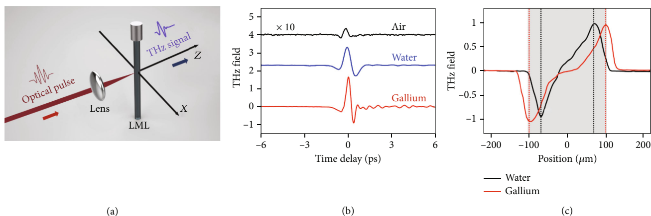
FIGURE 11: THz generation from liquid metal [71]. (a) Schematic of the experimental setup. A two-dimensional translation stage is used to control the position of the x -axis and the z -axis of the liquid metal line. The optical beam propagates along the z -axis. THz emission is measured by a standard electro-optical sampling. (b) Comparison of THz waveforms generated from air, water, and liquid gallium under single-color excitation. The target diameter is 210\ \mu\text{m} . The THz signal from air plasma is enlarged by 10 times. (c) Normalized THz field strength plotted as a function of the x -axis position. The dashed lines represent the x -axis position of the maximum THz fields. The gray area shows the diameter of the liquid line.
