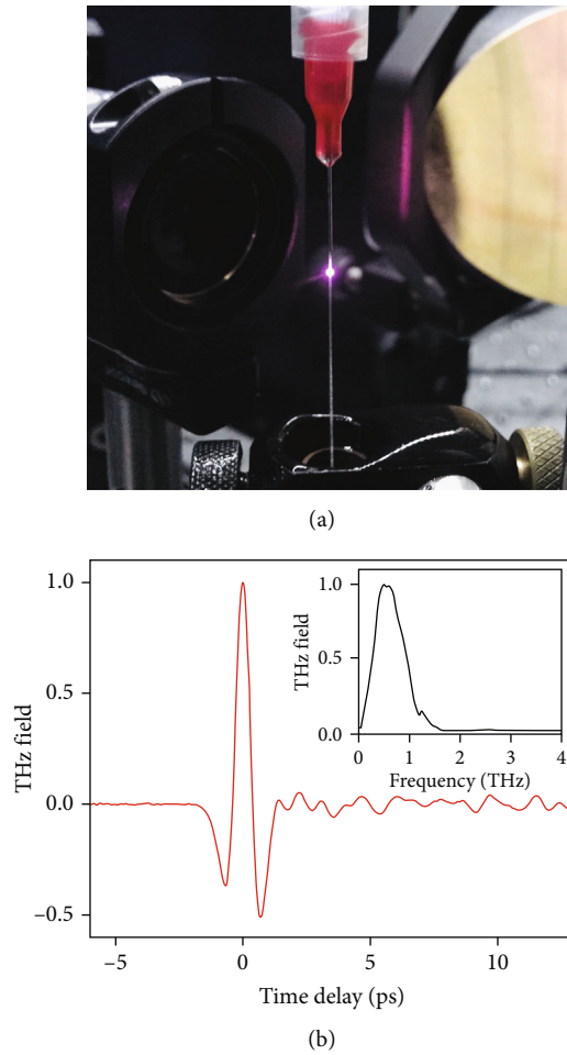
FIGURE 5: THz generation from liquid water under single-color ionization. (a) A photo of a fluorescence from a laser-induced microplasma of a water line. (b) A typical THz waveform generated from a water line and its corresponding spectrum (inset).
