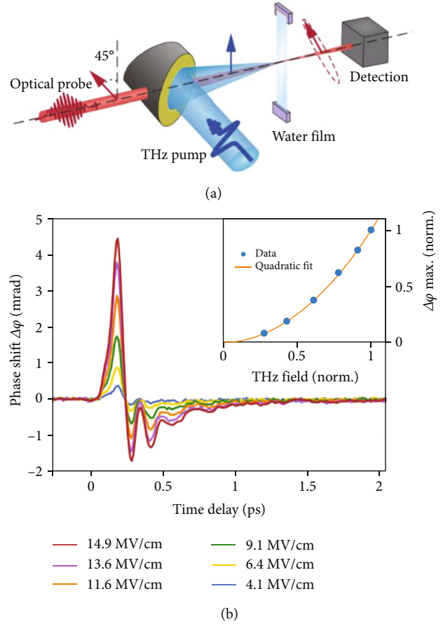
FIGURE 14: Terahertz Kerr effect (TKE) in a water film [85]. (a) Diagram of the experimental setup. An intense THz pulse generated from an organic crystal DAST (4-N, N-dimethylamino-4'-N'-methyl-stilbazolium tosylate) is focused onto a free-standing water film. The THz field-induced Kerr effect is detected by an optical probe. (b) TKE with different THz peak field strengths. Inset: THz field strength dependence.
