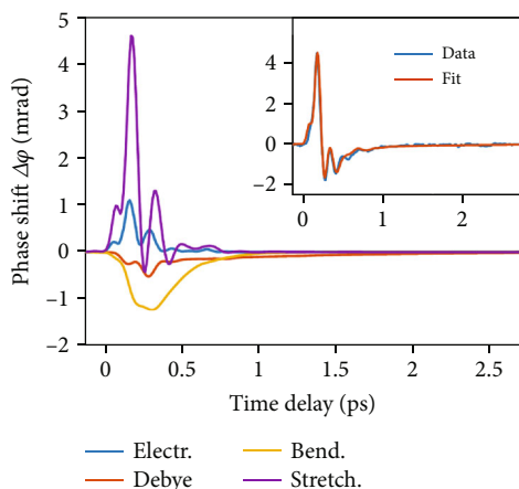
FIGURE 15: Simulation of the TKE response [85]. The simulation results of the TKE response in the time domain for the electronic (Electr.), Debye relaxation (Debye), hydrogen bond bending vibration (Bend), and hydrogen bond stretching vibration (Stretch.) contributions. Inset: a comparison between the sum of the fitted contributions and the measured data.
