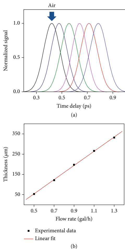
FIGURE 3: Calibration of the water film thickness. (a) The original (air) signal from the autocorrelation system is plotted in the black line. With the water film inserted in one of the two laser beams of the autocorrelation system, the signal peak will move linearly with the increase of film thickness. (b) The linear dependence of the film thickness on the flow rate. The thickness of the water film can be continuously varied from 50 \mu\text{m} to 350 \mu\text{m} .
