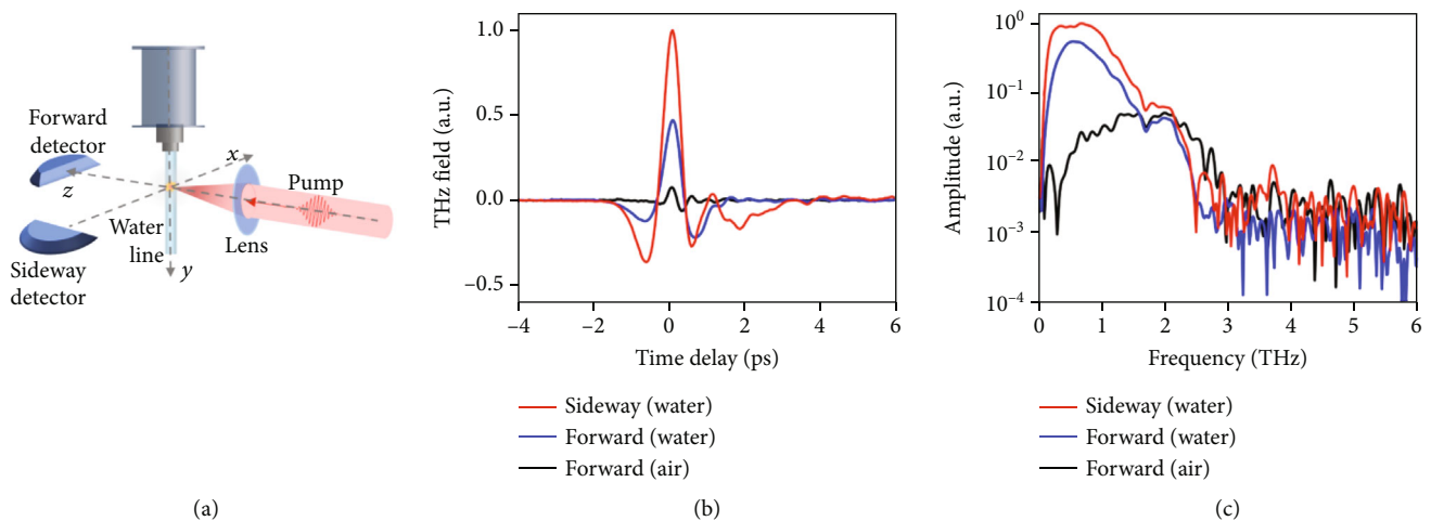
FIGURE 8: Comparison of forward and sideways detection. (a) Setup schematic for forward and sideways detection. The pump beam is along the z -axis. The water line flows in the y direction. Two EO detectors are in the z and x directions. (b) Comparison of THz waveforms. The laser pulse energy is 0.4 mJ. Corresponding spectra are shown in (c).
