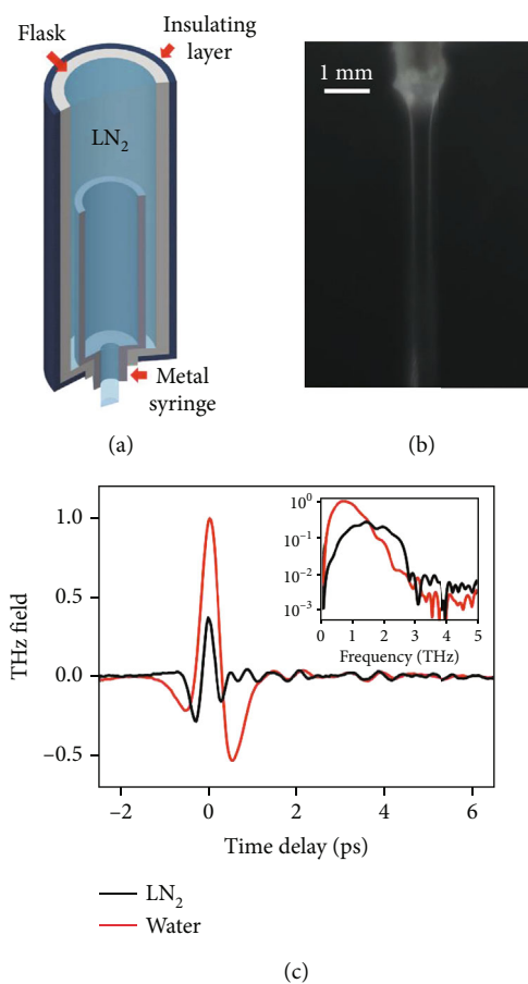
FIGURE 10: THz generation from liquid nitrogen [67]. (a) Diagram of the apparatus for guiding an \text{LN}_2 line. By filling it with \text{LN}_2 , the liquid in the flask prevents the liquid in the syringe transferring heat. (b) A photo of a flowing \text{LN}_2 line in an ambient environment. The transparency of the line indicates the liquid phase clearly with a smooth surface. (c) Comparison of THz waveforms from water and \text{LN}_2 under the same optical excitation. Inset: corresponding spectra.
