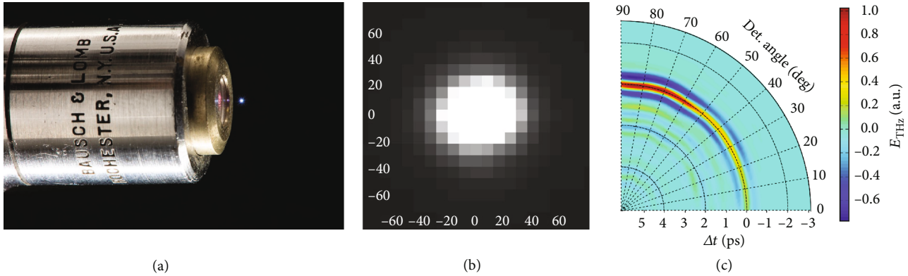
FIGURE 4: Microplasma and the signal distribution [34]. (a) A photo of the microplasma fluorescence obtained by focusing the laser beam with a high NA microscope objective. (b) A magnified image of the microplasma (unit is \mu\text{m} ). However, the plasma spot's contribution to the THz wave is about one micrometer or less. (c) Measured THz field as a function of the THz emission angle. The optimal angle is 80 degrees from the laser propagation direction.
