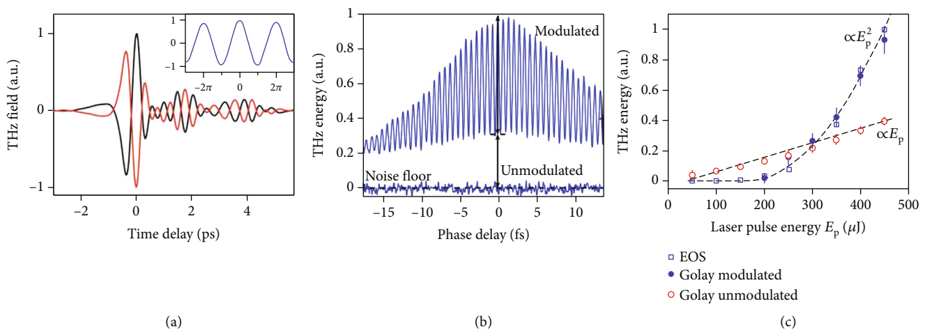
FIGURE 9: THz generation from liquid water under two-color excitation [13]. (a) Two THz waveforms are obtained when the relative phase is \pi and 2\pi . Inset: THz electric field as a function of the phase delay. (b) THz wave energy with a tuned phase between 800 nm and 400 nm pulses. The THz energy was monitored by a Goly cell. (c) Normalized THz energy from liquid water as a function of the total laser pulse energy. Blue squares show the THz energy calculated from the temporal integral of the THz waveform measured by the EOS. Blue dots indicate modulated THz energy measured by a Goly cell. Red circles present unmodulated THz energy measured by the Goly cell.
