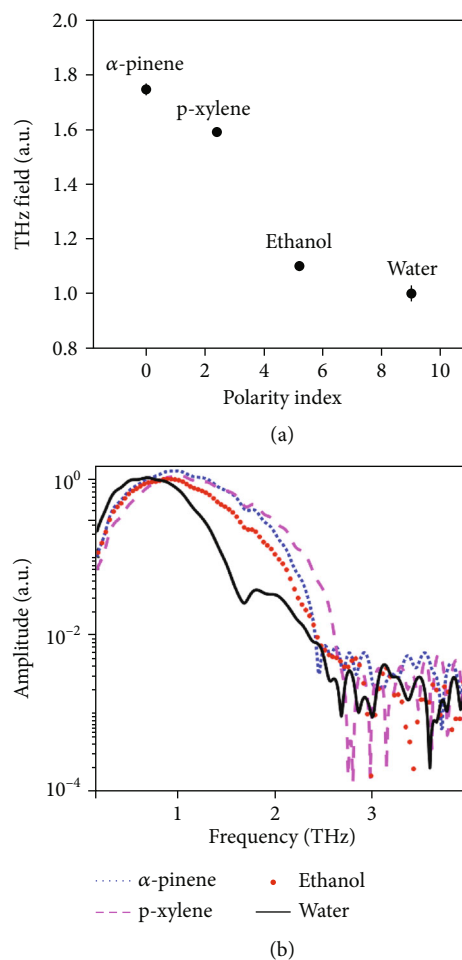
FIGURE 12: THz generation from liquids with different polarity indices. (a) THz fields generated from four liquids, which are \alpha -pinene, p-xylene, ethanol, and water. Their polarity indices are 0, 2.4, 5.2, and 9, respectively. (b) Corresponding spectra.
