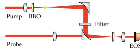
FIGURE 1: A typical THz two-color air plasma system. The laser beam is split into the pump beam and probe beam. The air plasma is produced by focusing the pump beam. One BBO crystal is inserted to create the second harmonic pulse. The THz signal is detected via electro-optic sampling (EOS).
