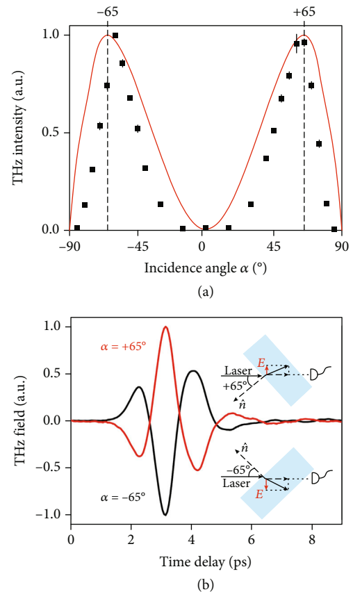
FIGURE 6: The dependence of the THz signal on the incidence angle \alpha [10, 12]. (a) THz intensity with different incidence angles is studied by rotating the water film. The THz signal is maximized when \alpha is 65^\circ . The squares are the experimental results, and the red line is a simulated result from a dipole model. (b) Two THz waveforms obtained with opposite incident angles. The insets explain the observation with a contribution of the flipped dipole projection ( E ) of opposite incidence angles.
