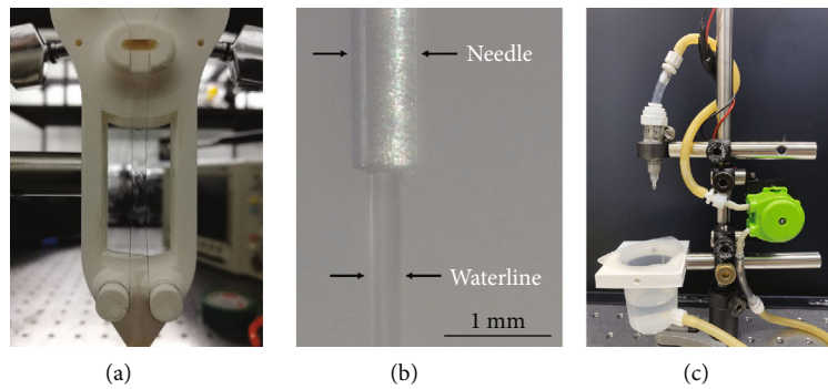
FIGURE 2: Liquid targets and the liquid system. (a) A gravity-driven water film. The thickness is 210\ \mu\text{m} . (b) A pump-driven water line with a diameter of 260\ \mu\text{m} , which is guided by a syringe needle. (c) A home-built liquid system, which needs only 50 ml water for several hours running. A syringe is used as a jet for producing a liquid line.
