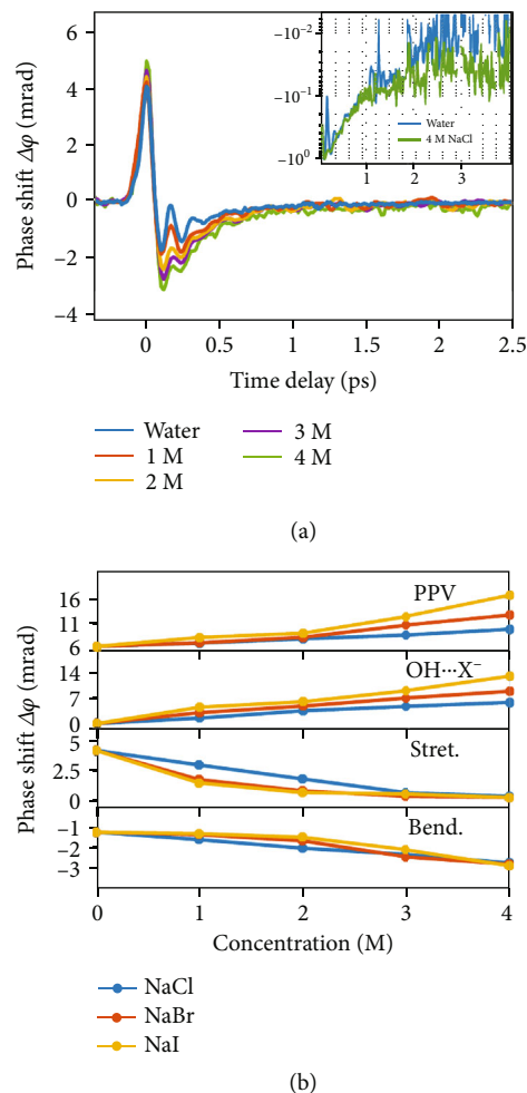
FIGURE 16: Terahertz Kerr effect response on different concentrations [89]. (a) TKE responses of water and NaCl solutions in different concentrations. Inset: an enlarged logarithmic view of the negative polarity responses. (b) The upper panel shows the measured peak-to-peak values (PPV) of TKE responses for NaCl, NaBr, and NaI solutions in different concentrations. The other panels show the extracted maximum values of TKE responses induced by \text{OH}\dots\text{X}^- hydrogen bond vibration ( \text{OH}\dots\text{X}^- ), the hydrogen bond stretching modes (Stret.), and the hydrogen bond bending (Bend.).
