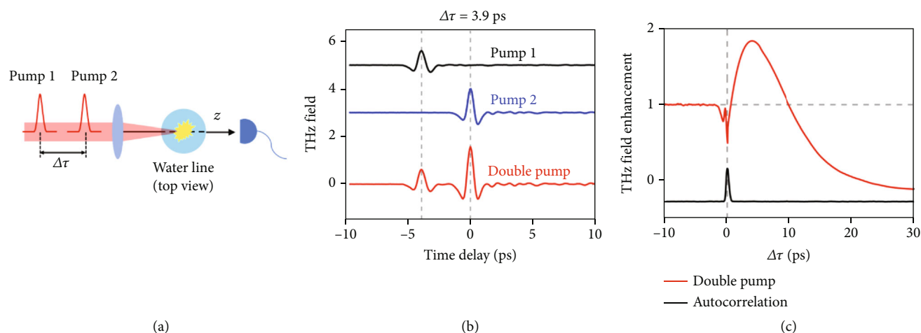
FIGURE 13: THz generation under double-pump excitation [79]. (a) Schematic of double-pump excitation. Two optical pumps propagating collinearly with a certain time delay \Delta\tau are focused on a water line (top view). \Delta\tau is controlled by a delay stage. The THz signal is detected via EOS. (b) THz waveforms generated by pump 1 (black line) and pump 2 (blue line). The bottom red line shows the waveform generated by two pumps when \Delta\tau is 3.9 ps. (c) The red line shows the dynamic enhancement of the THz peak field versus \Delta\tau . The black line plots the autocorrelation signal of the two pumps, from which the 0 timing is determined. \Delta\tau > 0 means that the pump 1 ionizes the target first.
