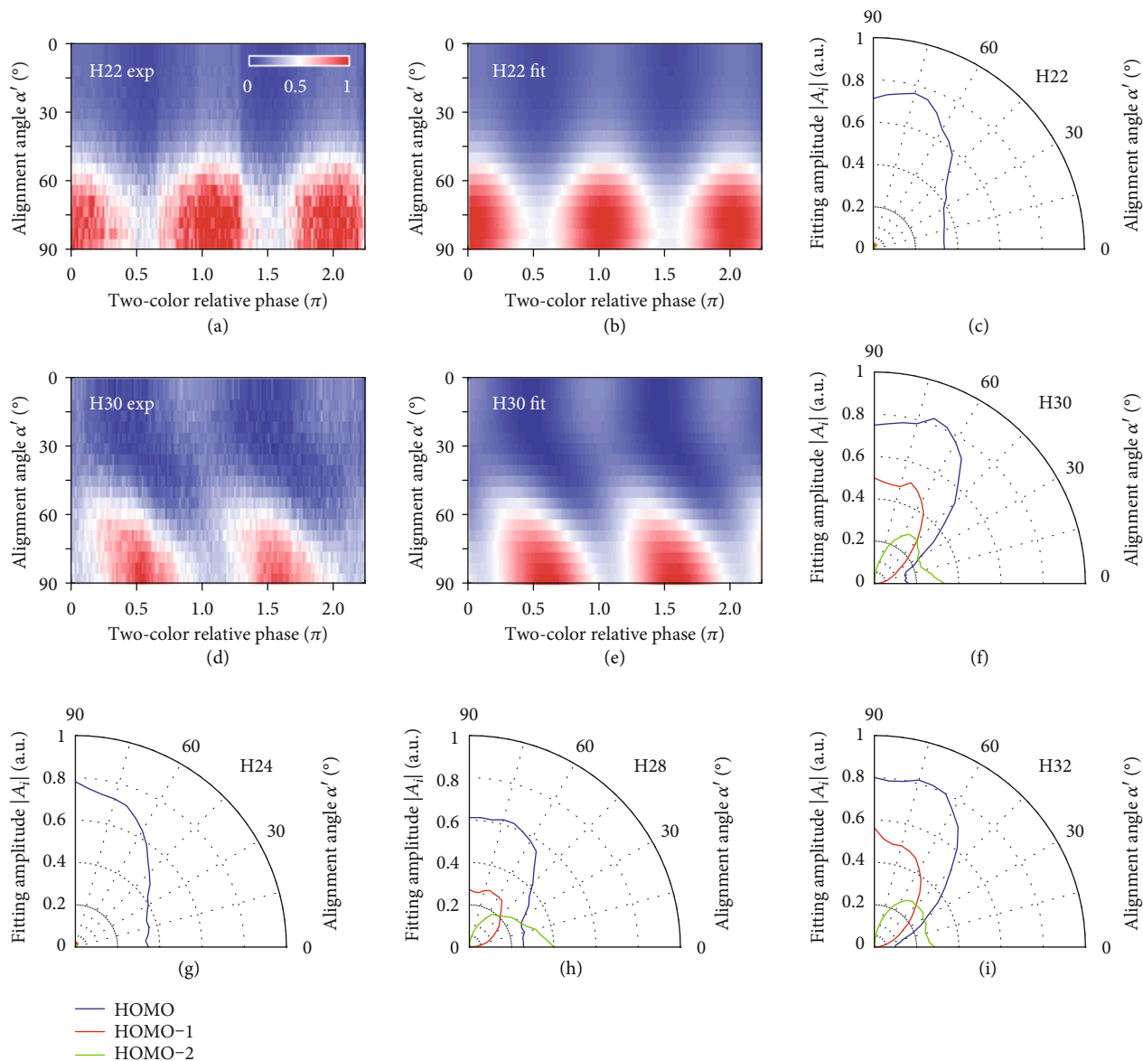
FIGURE 4: Fitting the participation of different orbitals. Experimental (a) and fitting (b) yields of H22. (c) The fitting amplitudes of HOMO (blue lines), HOMO-1 (red lines), and HOMO-2 (green lines) for H22, shown in polar coordinate. (d–f) present the same for H30. For comparison, we present the fitting amplitudes of the three molecular orbitals for H24 (g), H28 (h), and H32 (i). The standard deviation of the fitting amplitudes |A_i| is estimated to be less than 5%.
