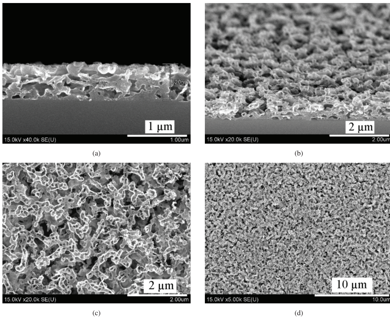
Fig. 1. SEM images of a porous nanostructured film formed on monocrystalline silicon containing seven layers of strontium titanate xerogel: (a) Cleaved edge. (b) Image taken at an angle of 70 to the sample surface. (c, d) Images of the surface at different magnifications.
