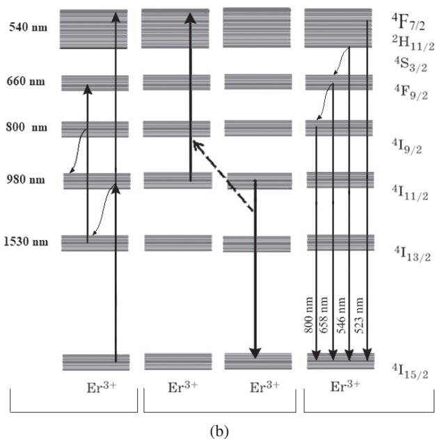
Fig. 5. (a) Upconversion luminescence spectra of (BaTiO 3 :Er)/SrTiO 3 /Si sample for the excitation wavelength 980 nm of a 200 mW diode module after annealing of each layer of BaTiO 3 :Er at 450°C and final annealing at 800°C or 900°C. (b) Scheme of upconversion luminescence of Er 3+ ions with separation the excited state absorption (left), energy transfer upconversion between two neighboring ions (middle) and transitions from the excited states (right).
