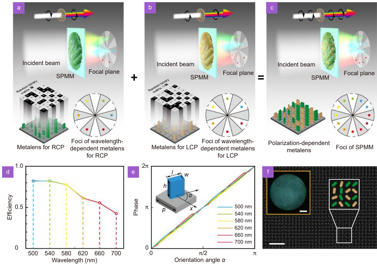
Fig. 2 | Design and realization of the SPMM. (a, b) The metalenses designed for RCP (or LCP) based on the holography principle possess six working wavelengths and six corresponding off-axis foci at different positions on the same focal plane. (c) The SPMM with twelve different foci was acquired by mixing nanostructures of these two metalenses together randomly. (d, e) The simulated cross-polarization conversion efficiencies (d) and phase retardation (e) corresponding to six discrete wavelengths. The materials of the nanostructure and substrate were \text{SiN}_x and \text{SiO}_2 , respectively. h=600 nm, w=130 nm, l=323 nm, and p=450 nm. (f) The SEM images of the fabricated metasurface (scale bar 2 \mu\text{m} ). The fake color represents randomly mixed nanostructures. An optical inset shows the whole SPMM, which is 500 \mu\text{m} in diameter (scale bar 50 \mu\text{m} ).
