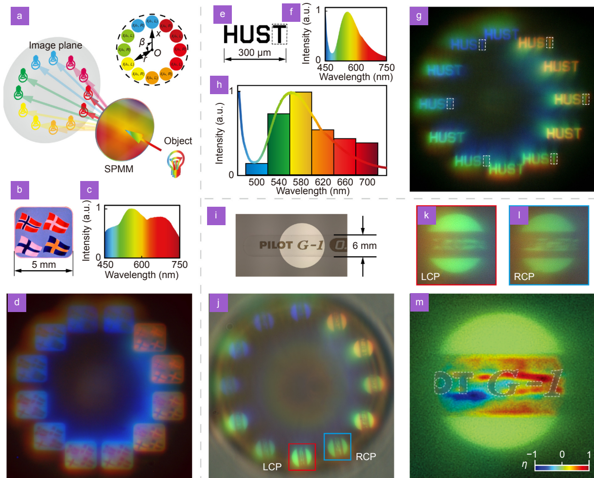
Fig. 5 | Multispectral and polarized imaging using the SPMM with ordinary white light beams. (a) Schematic illustration of the experiment. (b–d) Imaging results for a color picture consisting of four flags. The light source is a halogen lamp, and its spectrum is presented in (c). (e–g) Imaging results for the phrase "HUST", with the spectrum of a mobile phone flashlight that was used as the light source. (h) Histogram of the reconstructed spectra based on six regions marked with dash lines in (g). (i, j) Regular optical image and the SPMM imaging results for a transparent plastic stick. (k, l) A pair of typical images with the same spectral band are enlarged. (m) The reconstructed polarization ellipticity image can be calculated from the SPMM imaging results in (j). The images of corresponding opaque patterns are marked with dashed lines.
