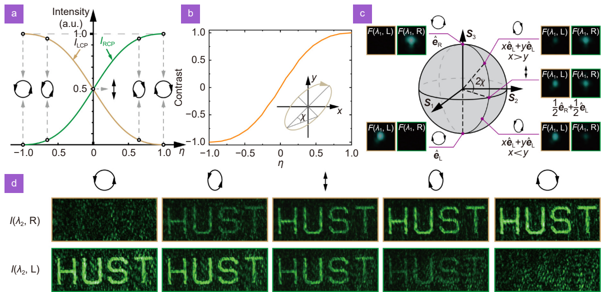
Fig. 4 | Polarization-dependent focusing and imaging using the SPMM. (a) The relationship between normalized intensities I_{RCP} (or I_{LCP} ) of RCP (or LCP) light and the polarization parameter \eta in the Jones matrices. (b) The contrast calculated by (I_{RCP}-I_{LCP})/(I_{RCP}+I_{LCP}) . (c) Typical polarization state measurement results at 500 nm, with the polarization state of the incident light beam varied gradually from LCP to RCP. The intensity of the focus at position F (500 nm, R) increases from zero to maximum, with this trend reversed at F (500 nm, L). (d) Imaging results achieved by the SPMM at a wavelength of 540 nm.
