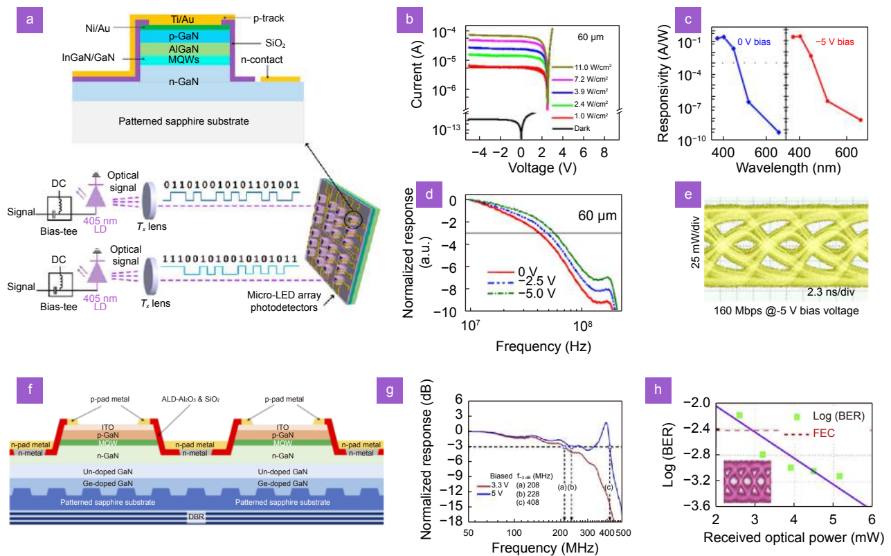
Fig. 10 | (a) Cross-section of the \mu LED and schematic setup for VLC system using the \mu LED based photodetectors. (b) Current–voltage ( I – V ) curves of the \mu LED-based PD with diameters of 60 \mu\text{m} under darkness and illumination. (c) Responsivities of the \mu LED-based PD measured for various laser wavelengths. (d) Frequency response for \mu LED-based PD. (e) Eye diagrams at a transmission rate of 160 Mbps. (f) Cross-section of semipolar green \mu LEDs. (g) Frequency responses of \mu LED PD. (h) BERs with \mu LEDs as PD at a transmission rate of 540 Mbps. Figure reproduced with permission from: (a–e) ref. 165 , American Chemical Society; (f–h) ref. 166 , under the OSA Open Access Publishing Agreement.
