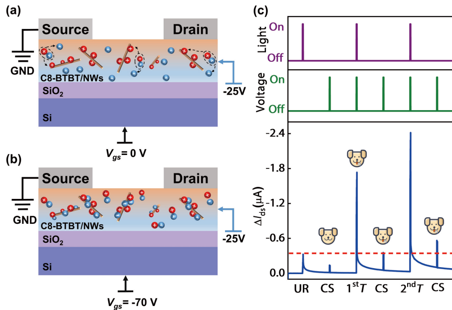
Fig. 4. (Color online) Schematic illustrations of (a) the existence of electrons in the device after light illumination and (b) the recombination process of electrons and holes with voltage applied to the gate. (c) The complete association learning process. After training, CS can trigger UR (canine saliva secretion, unconditional response).
