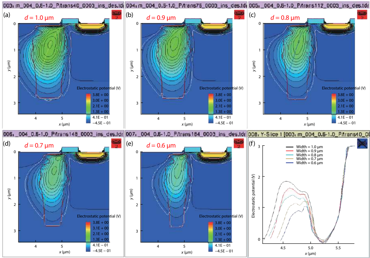
Fig. 6. (Color online) Potential and depletion region distribution with different single-finger PPD widths.
