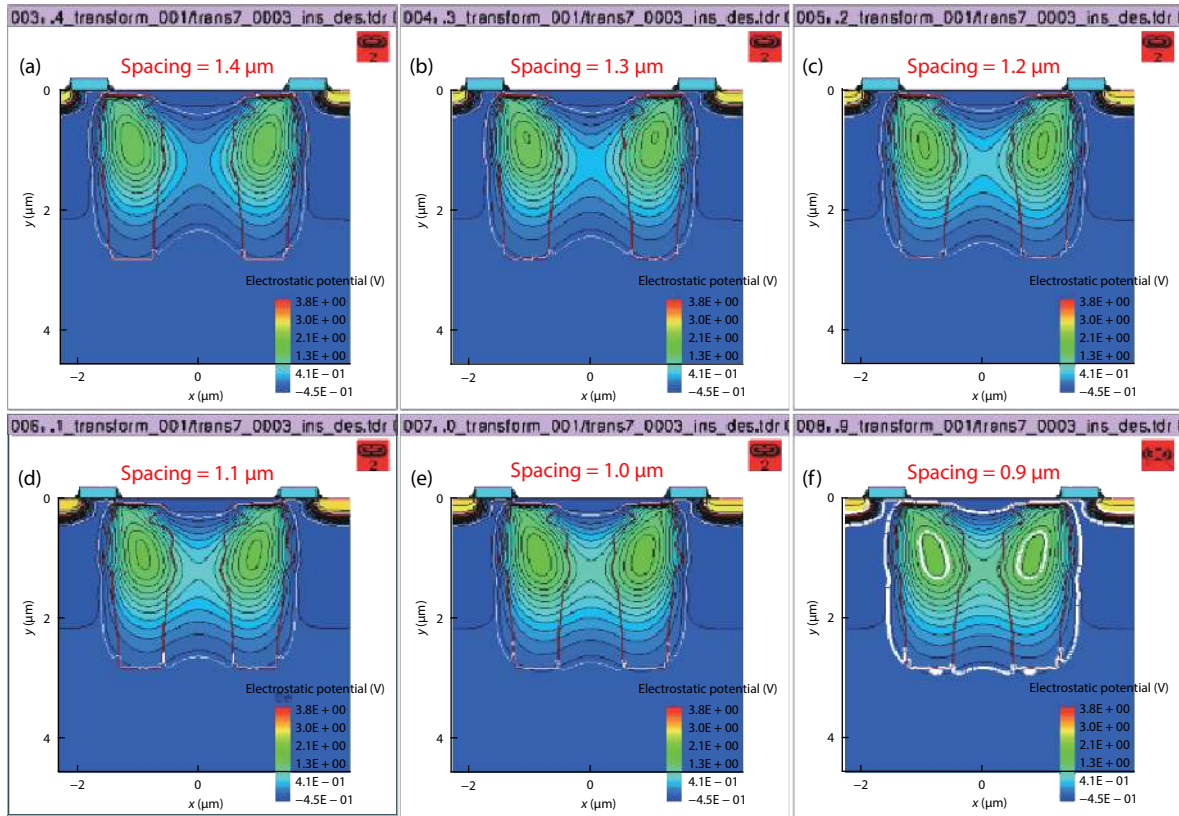
Fig. 8. (Color online) Depletion zone and potential distribution with different PPD spacing.
