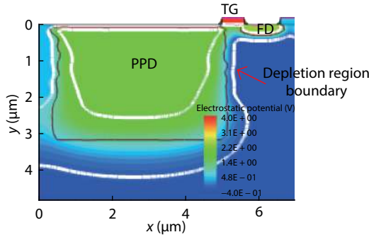
Fig. 2. (Color online) 2D TCAD simulation of depletion region in traditional cubic PPD.
