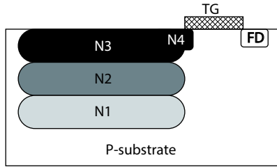
Fig. 1. N buried layer structure of PPD.
