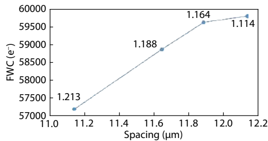
Fig. 13. (Color online) FWC with different spacing (Before widening N1).
