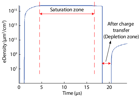
Fig. 7. (Color online) The number of electrons in PPD based on TCAD 2D simulation.
