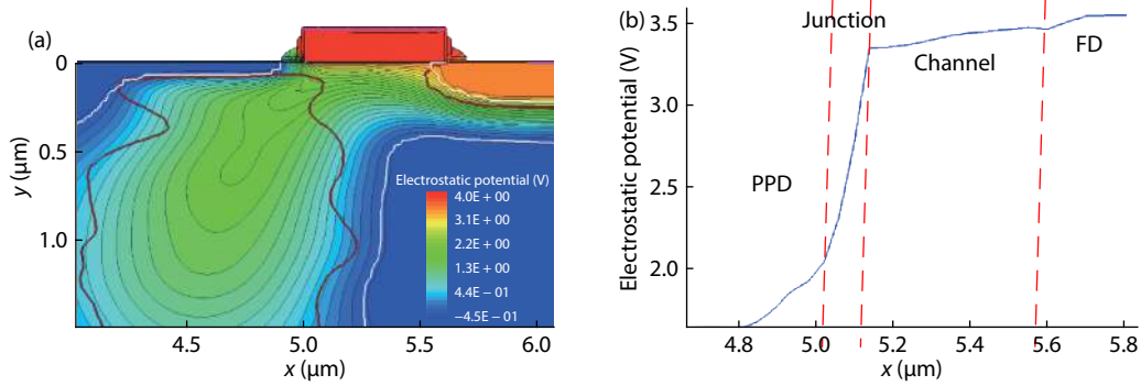
Fig. 5. (Color online) Under the basic ion implantation process conditions: (a) the potential distribution in transfer phase, (b) the potential curve on the charge transfer path.
