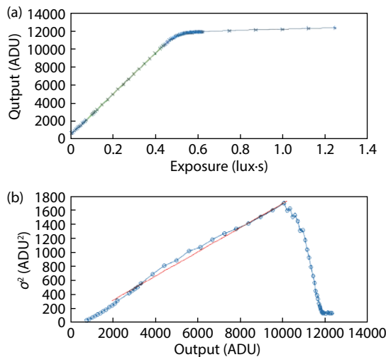
Fig. 14. (Color online) The measurement results of test chip: (a) photoreponse of the pixel using the proposed PPD structure, (b) PTC of the pixel using the proposed PPD structure.
