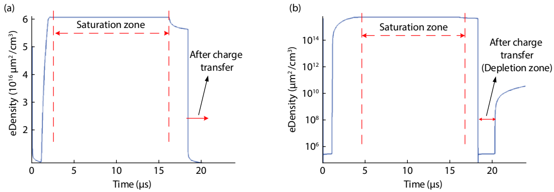
Fig. 9. (Color online) The number of electrons in PPD based on TCAD 2D simulation. (a) Using the process conditions of Fig. 2. (b) Using the process conditions of Fig. 8(d).
