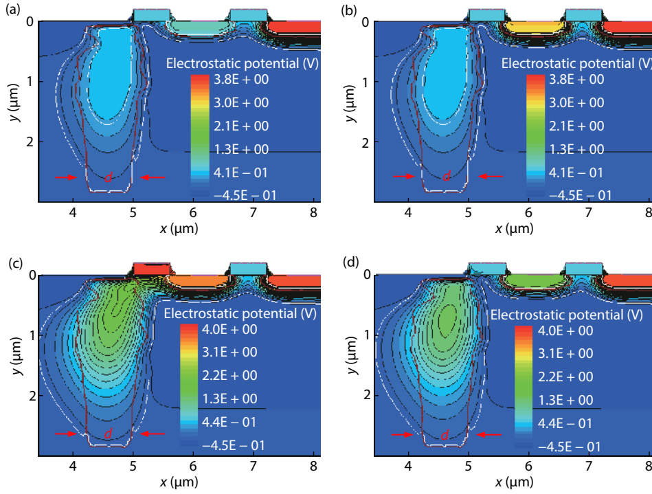
Fig. 4. (Color online) Under the basic ion implantation process conditions, the potential distribution in (a) initial phase, (b) after illumination phase, (c) transfer phase, (d) post-transition phase.
