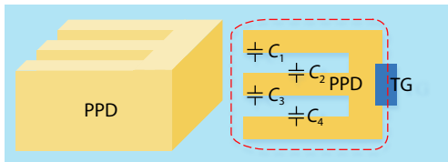
Fig. 3. (Color online) The finger-shaped PPD and its top view.
