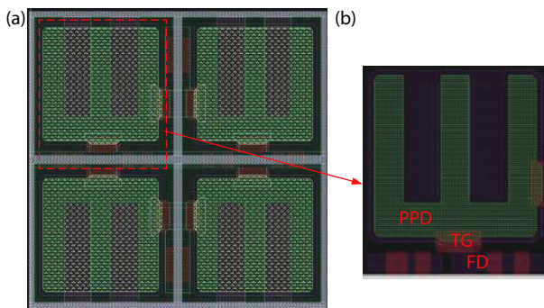
Fig. 11. (Color online) Pixel layout and the main layout level of PPD-TG-FD. (a) 2 × 2 pixel unit. (b) Layout of PPD-TG-FD.
