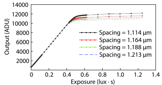
Fig. 12. Photoresponse with different single-finger spacing. with other imaging devices in Refs. [20–23]. It shows that the PPD structure proposed in this paper effectively improves the full well capacity of CIS.
