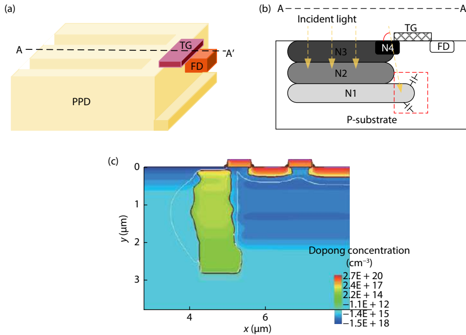
Fig. 10. (Color online) The special finger-shaped PPD structure proposed in this paper: (a) three-dimensional structure, (b) sectional structural view, (c) 2D device simulation diagram.
