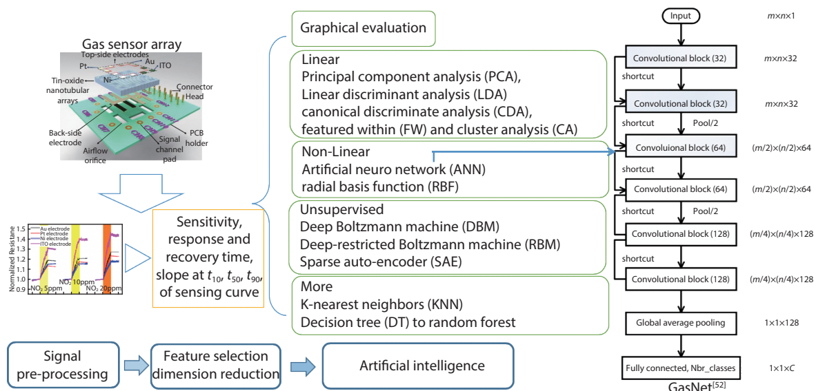
Fig. 4. (Color online) Artificial intelligence algorithms adopted in a gas sensor array.
