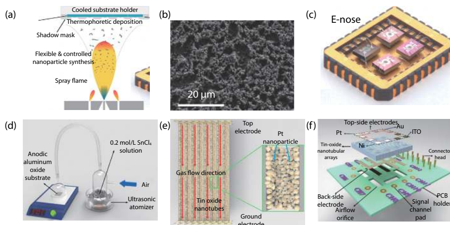
Fig. 2. (Color online) MOX sensor array fabrication method and morphology [10, 11] : (a) FSP set-up, (b) SEM image of porous doped SnO 2 film, (d) USP setup, (e) Cross-section of SnO 2 nanotube decorated with Pt nanoparticles, gas sensor array of (c) doped SnO 2 microsensors and (f) 3-D SnO 2 nanotube.
