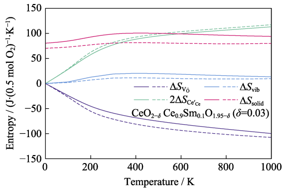
Fig. 4 Variations of \Delta S_{V\delta} , 2\Delta S_{Ce'Ce} , \Delta S_{vib} , and \Delta S_{solid} with temperature. Solid and dash curves are for CeO_2/CeO_{2-\delta} and Ce_{0.9}Sm_{0.1}O_{1.95}/Ce_{0.9}Sm_{0.1}O_{1.95-\delta} redox pairs ( \delta=0.03 ), respectively; Colourful figure is available on website
