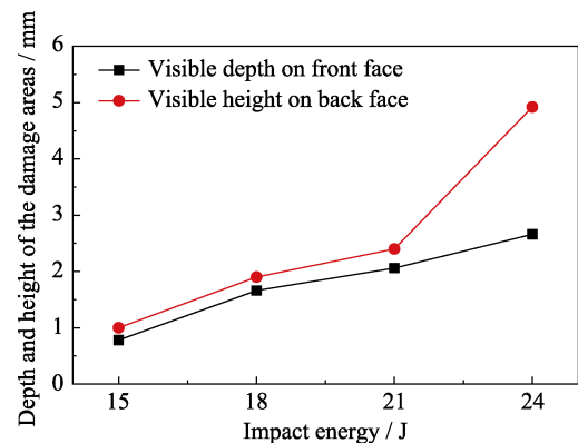
图 7 不同能量冲击后材料的正面凹坑深度及背面凸起高度 Fig. 7 Depth and height of the damage areas for the composites after impact with different energies
