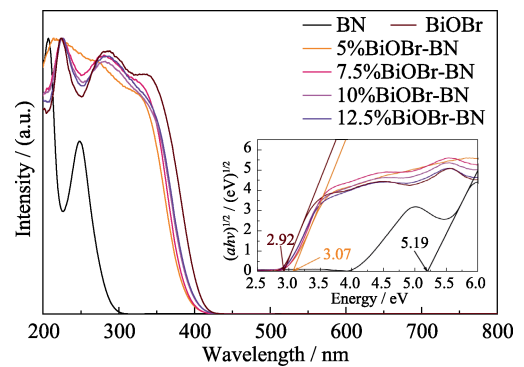
图 S9 BiOBr、BN 和 BiOBr-BN 复合样品的紫外-可见漫反射光谱 Fig. S9 UV-Vis diffuse reflectance spectra of BiOBr, BN and BiOBr-BN nanocomposites
