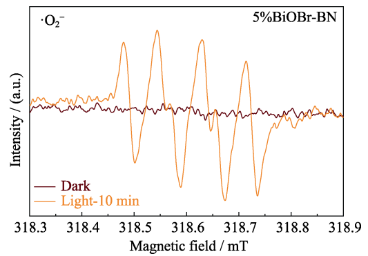
图 10 5%BiOBr-BN 样品的 DMPO(DMPO·O 2 - )捕获自由基的 ESR 光谱 Fig. 10 DMPO spin-trapping ESR spectra recorded with 5%BiOBr-BN in methanol dispersion for DMPO·O 2 -
