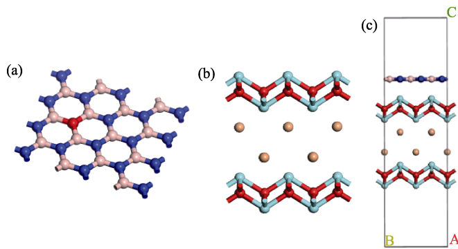
图 S8 BiOBr-BN 结构计算模型 Fig. S8 Model structure of BiOBr-BN (a) BN; (b) BiOBr; (c) BiOBr-BN
