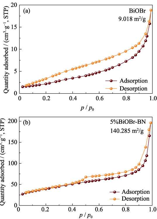
图 8 (a)BiOBr 和(b)5%BiOBr-BN 的氮气吸脱附等温曲线 Fig. 8 Nitrogen absorption-desorption isotherms of (a) BiOBr and (b) 5%BiOBr-BN
