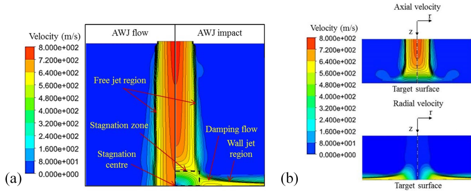
Figure 9. Comparison of velocity contour of a free flow AWJ and an impacting AWJ (a), and velocity component contours of an impacting AWJ (b) ( S_d = 3 mm, U = 800 m s -1 and d_n = 0.76 mm).
