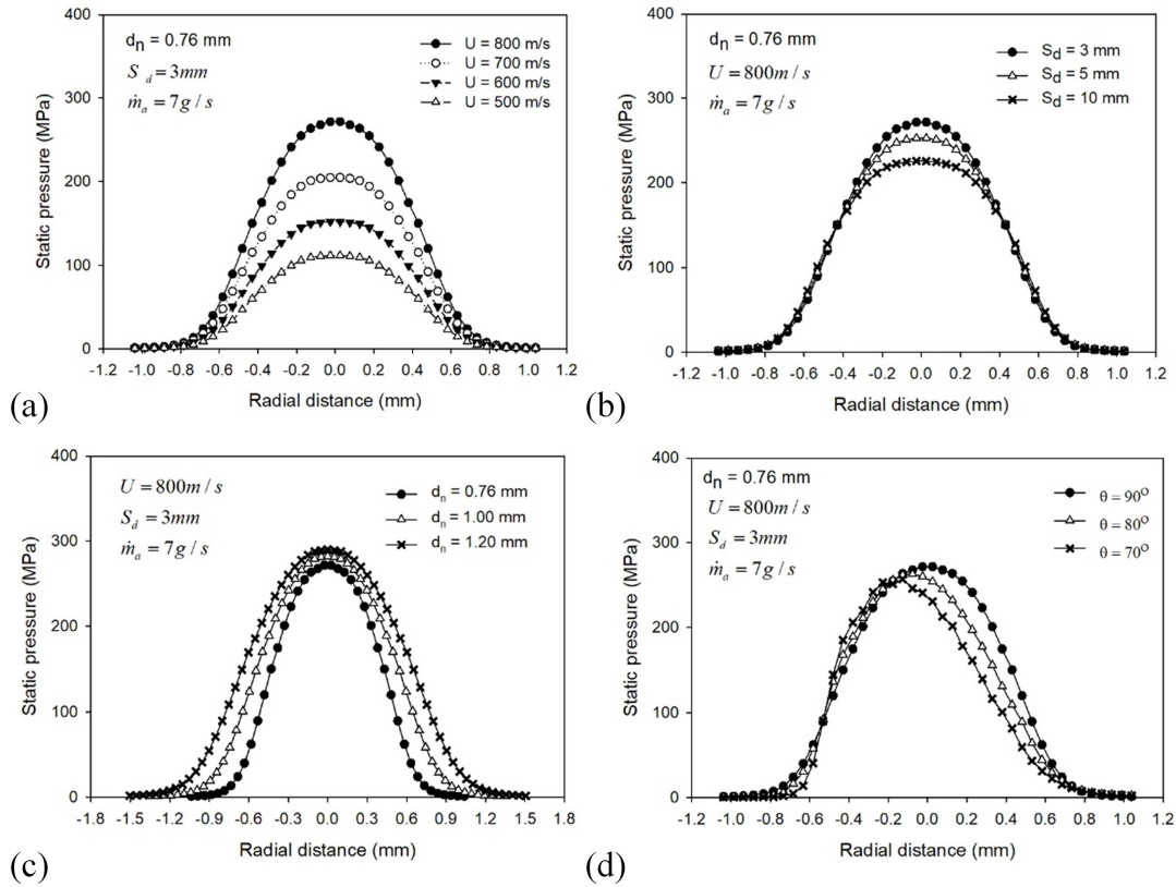
Figure 12. Static pressure on the target surface at different jet radial locations and under different impact conditions.
