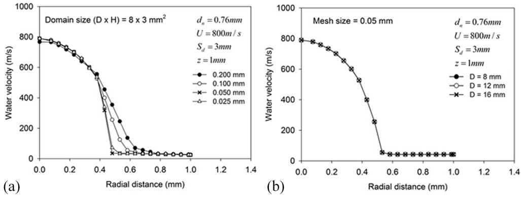
Figure 2. Calculated water velocity profile in the jet radial direction under: (a) different mesh sizes and (b) different domain sizes.
