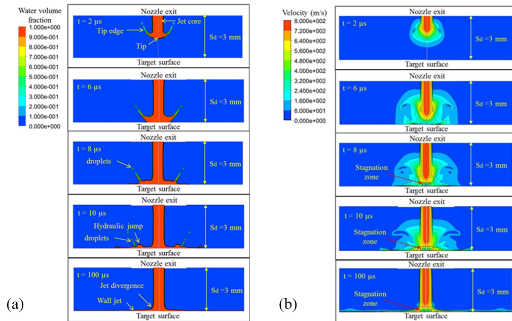
Figure 8. Evolution of an AWJ impact process with time: (a) water volume fraction contour and (b) water velocity contour ( S_d = 3 mm, U = 800 m s -1 and d_n = 0.76 mm).
