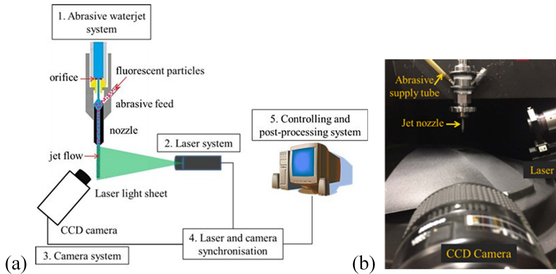
Figure 5. Experimental setup for particle velocity measurement: (a) schematic of the setup, and (b) actual setup.
