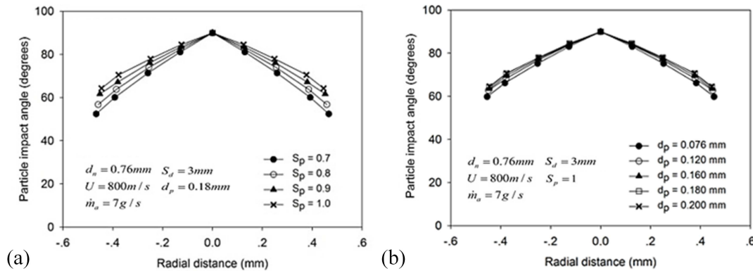
Figure 21. Effects of particle sphericity and particle diameter on particle impact angles.
