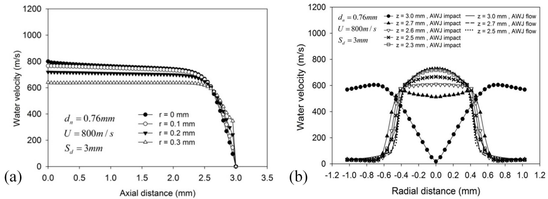
Figure 10. Waterjet velocity profiles: (a) in the jet axial direction and (b) in the jet radial direction.
