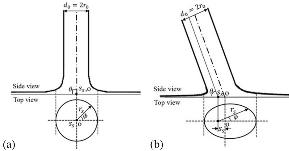
Figure 13. Schematic diagram of jet impingement area: (a) a perpendicular impact and (b) an oblique impact.
