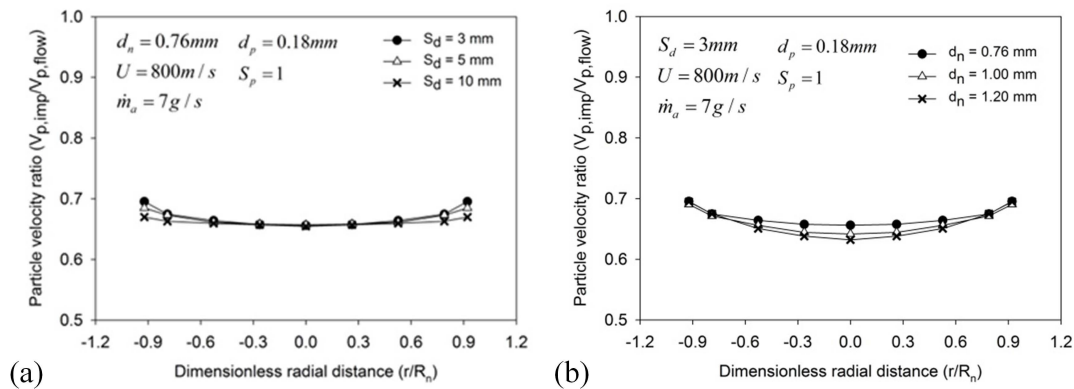
Figure 18. Variation of particle velocity ratio along the dimensionless jet radial direction under different: (a) standoff distances, and (b) nozzle diameters.
