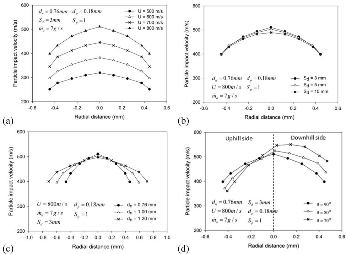
Figure 16. Particle velocity variation in the jet radial direction under different conditions.
