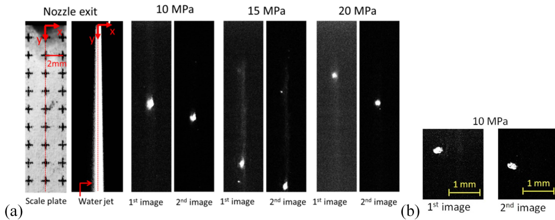
Figure 6. Image pairs of particle displacement (a), and particle translation and rotation (b).
