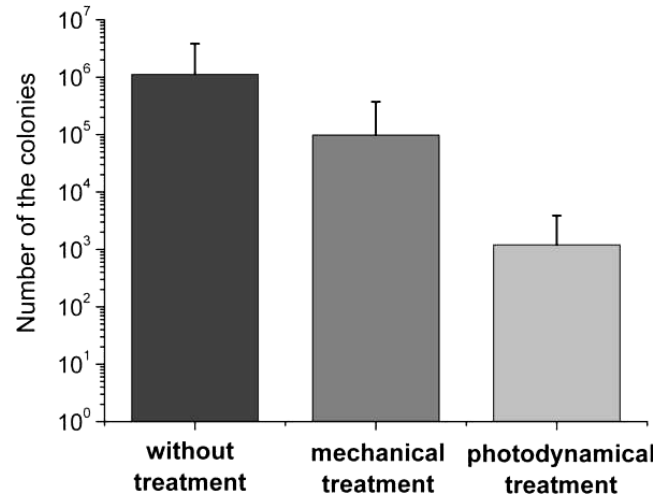
Fig. 3. Average value of in vitro measured bacterial colony forming rate (number of the colonies) of bacteria taken from tooth plaque: without treatment (control), after mechanical and photodynamical treatments.
