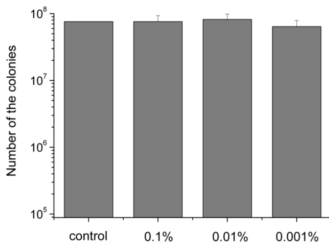
Fig. 2. Average value of in vitro measured bacterial colony forming rate (number of the colonies) of bacteria taken from tooth plaque after exposure to MB solution. The first column corresponds to control sample (without staining); the second, third and fourth columns to 3-min duration of 0.1%, 0.01%, and 0.001% MB solution action, respectively.
