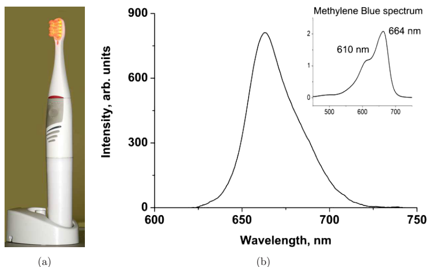
Fig. 1. R-LETB in a charger (a) and the emission spectrum of the R-LETB (b). Insert shows absorption spectrum of MB rinse solution.
