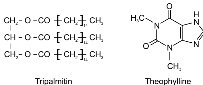
Fig. 1. Molecular structure formula of the lipid tripalmitin and drug theophylline.
