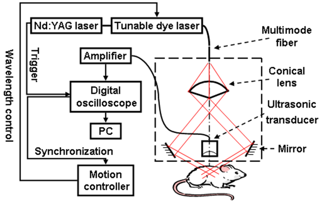
Fig. 1. Schematic of the dual-wavelength photoacoustic microscopy system.
