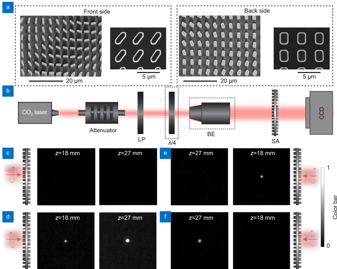
Fig. 4 | Experiment for the asymmetric transmission metasurface doublet. (a) SEM images for the front (left) and back (right) side of the metasurface. (b) Schematic illustration of the measurement setup. LP: linear polarizer. \lambda/4 : quarter wave plate. BE: beam expander. SA: sample. (c–f) Intensity distributions at z=18 mm and z=27 mm. (c) Front RCP incidence. (d) Front LCP incidence. (e) Back RCP incidence. (f) Back LCP incidence.
