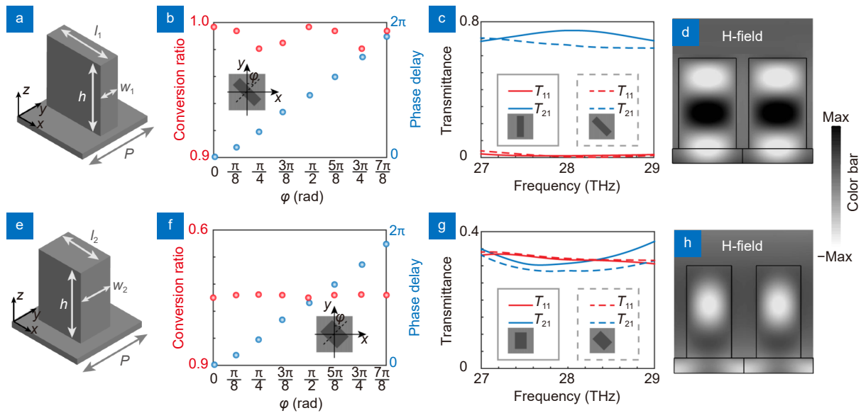
Fig. 2 | Unit cells for the CNOT LG metasurface doublet. (a, e) Schematic for HHWP and LHWP unit cells, respectively. P=4.5 \mu\text{m} , h=6 \mu\text{m} , l_1=3.7 \mu\text{m} , w_1=1.2 \mu\text{m} , l_2=2.9 \mu\text{m} and w_2=2.05 \mu\text{m} . (b, f) Corresponding polarization conversion ratio (left panel) and phase delay (right panel) with different \varphi for cross-polarized waves at 28.3 THz under LCP incidence. (c, g) Corresponding transmittance at \varphi=0 (solid lines) and \varphi=\pi/4 (dashed lines) from 27–29 THz. (d, h) Corresponding magnetic field distributions at \pm 28.3 THz.
