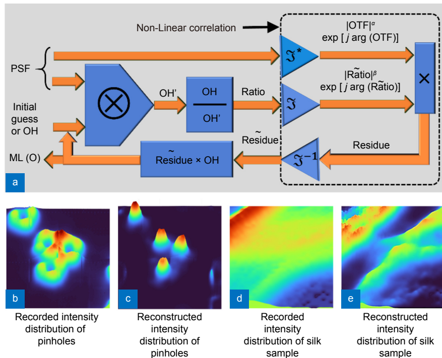
Fig. 2 | (a) Lucy–Richardson–Rosen algorithm. O: object; OH: object hologram, also used as the initial guess solution R^1 ; PSF: point spread function; OTF: – optical transfer function; \times : element by element product; \otimes : 2D convolution; \mathcal{F} : Fourier transform; \mathcal{F}^* : complex conjugate operation following a Fourier transform; \mathcal{F}^{-1} : inverse Fourier transform; \sim : Fourier transform of a variable; R^n and R^{(n+1)} : – n^{\text{th}} and (n+1)^{\text{th}} solutions, respectively; and ML(O): maximum likelihood solution of the object. (b) Recorded image of pinholes and (c) its reconstruction using LRRRA. (d) Recorded image of silk sample and (e) its reconstruction using LRRRA.
