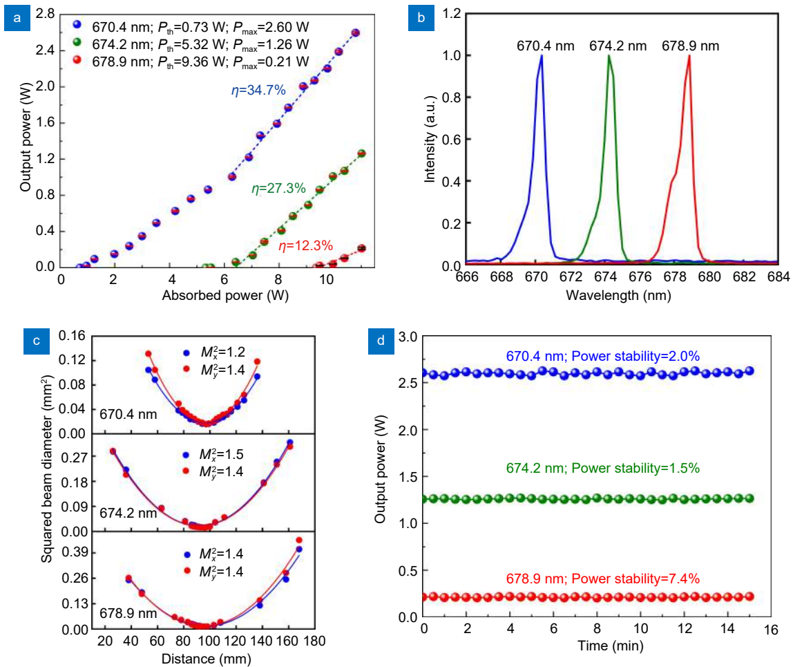
Fig. 2 | Experimental results of single-wavelength lasers around 670 nm. (a) Output powers and slope efficiencies with respect to absorbed pump powers. (b) Laser output spectra at 670.4 nm, 674.2 nm, and 678.9 nm, respectively. (c) Measured corresponding M^2 factors of 670.4 nm, 674.2 nm, and 678.9 nm, respectively. (d) Power stabilities of lasers at 670.4 nm, 674.2 nm, and 678.9 nm
