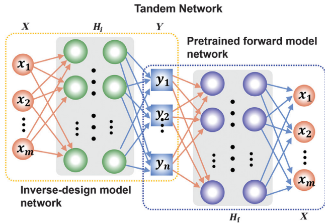
Fig. 2 The architecture of the TN model, which consists of an inverse-design network connected to a pretrained forward model network. X represents the input and output, which is the transmission spectra data in our case, and Y represents the output in the middle layer which is the structural parameters here.
