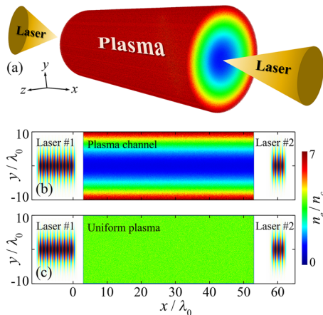
FIG. 1. (a) Schematic of the generation of collimated GeV positron jets by the interaction of two 10 PW laser pulses with a plasma channel filled with NCD plasma. The drive pulse (laser #1) and probe pulse (laser #2) are incident from the left and right sides, respectively. Two cases are considered: (b) a plasma channel with a radially symmetric density profile and (c) a uniform plasma slab.
