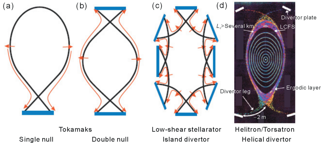
Fig. 5. Schematics of (a) single-null and (b) double-null tokamak divertors; and (c) the intrinsic island divertor for W7-X stellarator and (d) the helical divertor for LHD helitron [70].
