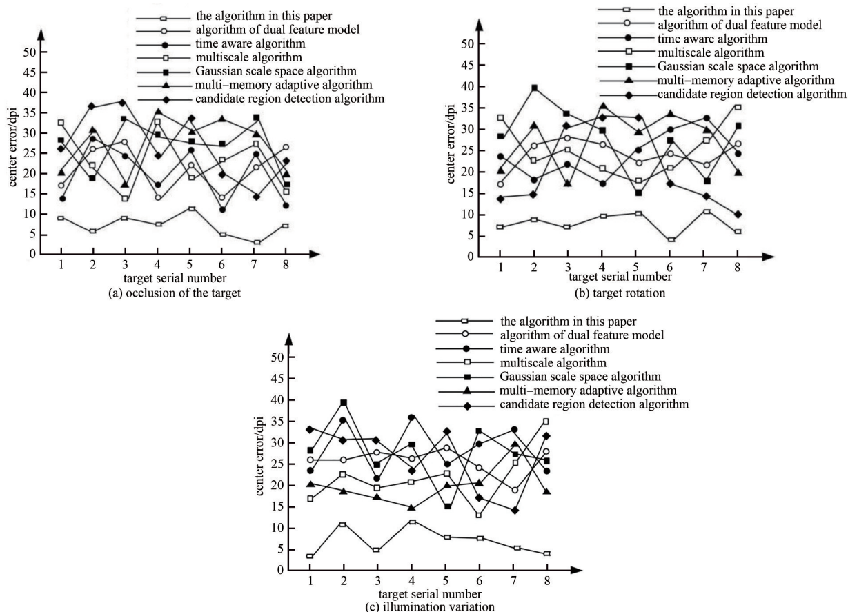
Fig.2 Center error comparison of different methods
