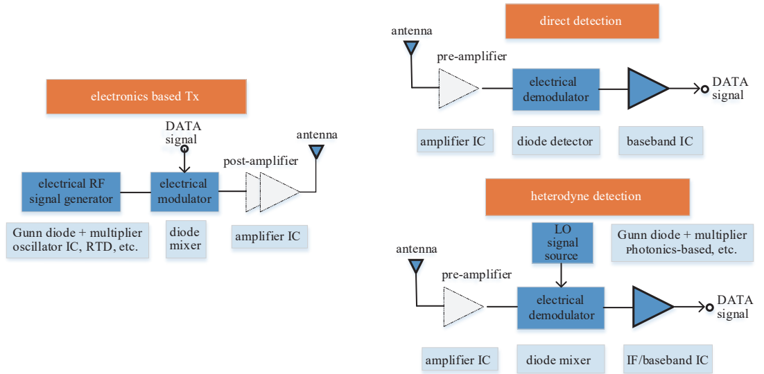
(a) Transceiver architecture of terahertz high speed wireless communication system based on all electronics
