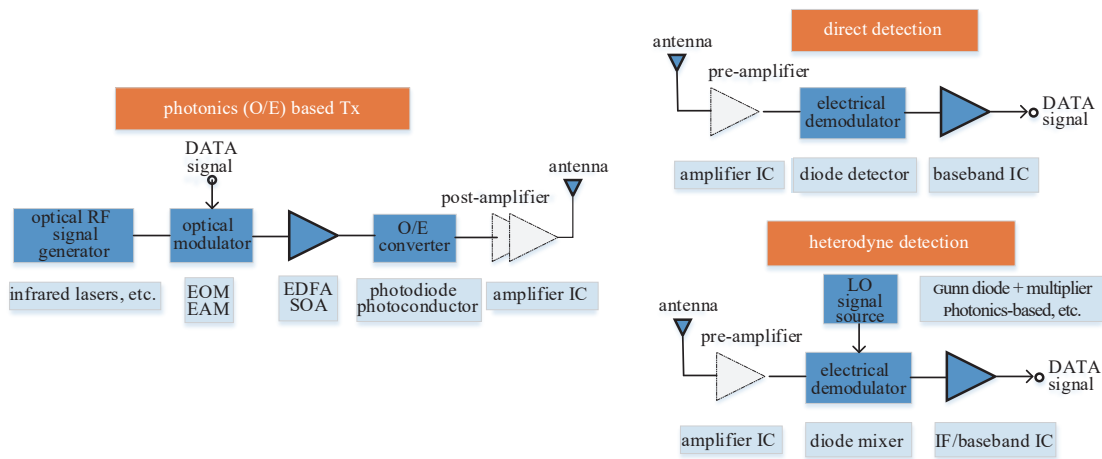
(b) Transceiver architecture of terahertz high speed wireless communication system based on photoelectric hybrid
