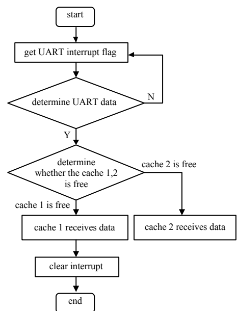
Fig.7 Flow chart of data interaction serial port interrupt 图 7 数据交互串口中断流程图
