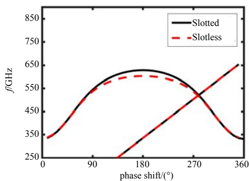
Fig.4 Influence of the slot structure on the dispersion 图 4 开孔对色散的影响
