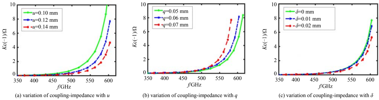
Fig.3 Impact of the dimensions of the slot-structure on the coupling-impedance 图 3 各参数对耦合阻抗的影响
