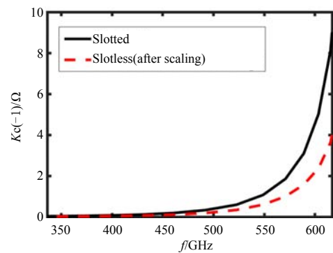
Fig.5 Influence of the slot structure on the coupling-impedance 图 5 开孔对耦合阻抗的影响
