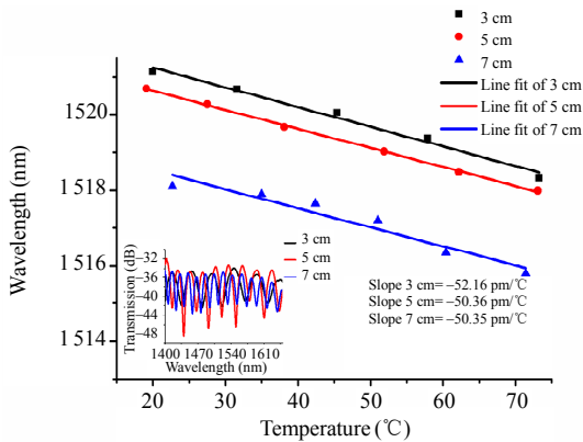
Fig. 5 Transmission spectrum based on the structure with different lengths of the FMF and measured temperature sensitivity.
