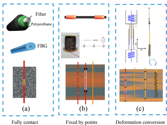
Fig. 15 Principle of deformation sensing with different measuring ranges: (a) 0–0.5%, (b) 0.5%–2%, and (c) 2%–50%.
