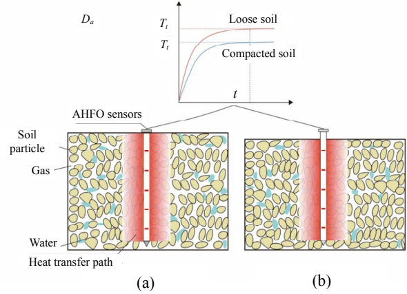
Fig. 10 Measurement principle of soil dry density: (a) loose soil and (b) compacted soil.
