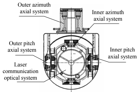
Fig. 1 Composition of the PAT system.
