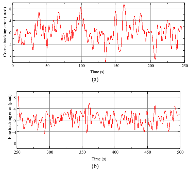
Fig. 8 Flight tracking precision test: (a) coarse tracking error and (b) fine tracking error.
