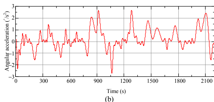
Fig. 5 Angular velocity (a) and the angular acceleration in coarse tracking (b).
