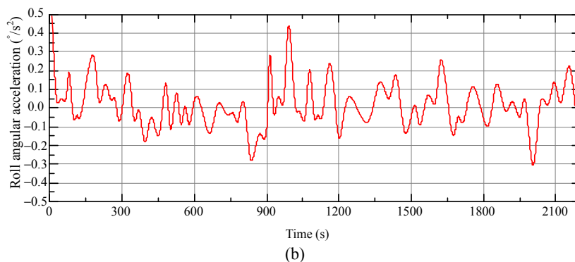
Fig. 6 Roll angular velocity (a) and the angular acceleration (b).
