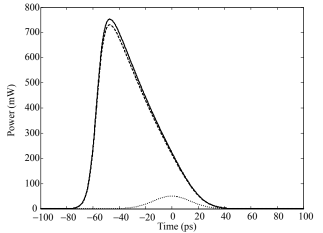
Fig. 1 Temporal profile of the input and output pulses: dotted line: the input pulse; dashed line: the analytical result by (20); the solid line: numerical result.
