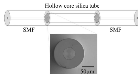
Fig. 2 Scheme of the sensor heads and a microscope image of the hollow core silica tube cross-section.
