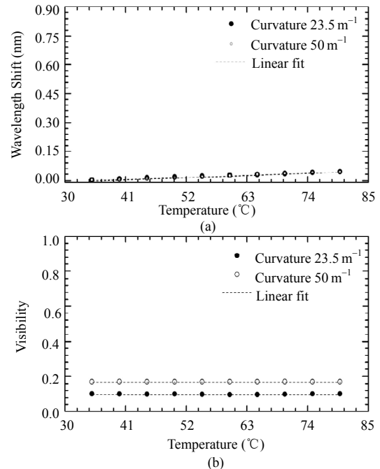
Fig. 6 Temperature characterization for FP-Long submitted to 23.5\text{m}^{-1} and 50\text{m}^{-1} of curvature applied (a) in wavelength and (b) in visibility.
