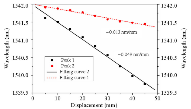
Fig. 3 Responses of dual-wavelength FBG to displacement.
