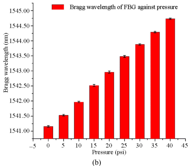
Fig. 7 Repeatability response of the FBG pressure sensor: (a) repeatability test results and (b) error bars of bar graph plotted between the FBG Bragg wavelength and pressure.
