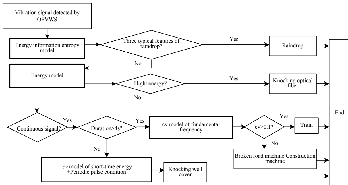
Fig. 6 Strategy for identifying vibration signals detected by OFVWS.
