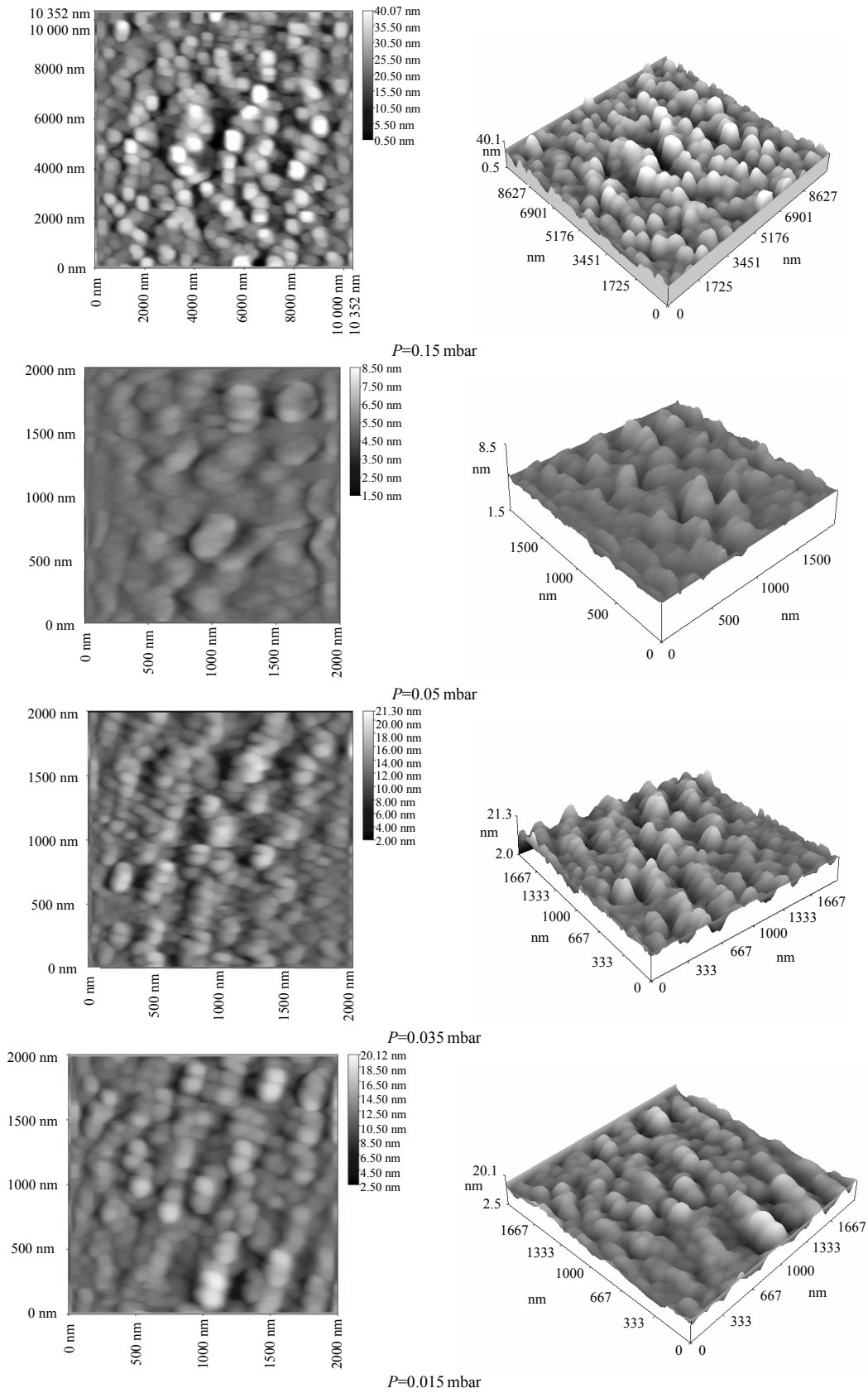
Fig. 2 AFM images of the sputtered SnO 2 thin films on glass substrates at different working pressures.
