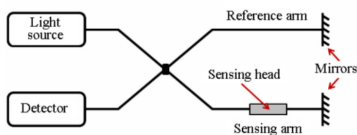
Fig. 2 Michelson fiber-optic interferometric configuration, consisting of a 2×2 coupler with 50:50 split, and with reflective elements (e.g. metallic mirror, FBGs, or other) added to the interferometer arms.
