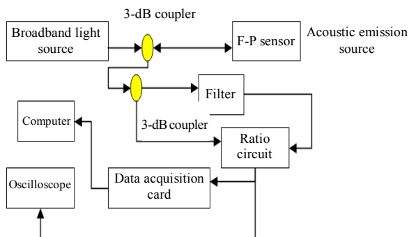
Fig. 2 Acoustic emission sensor monitoring system.
