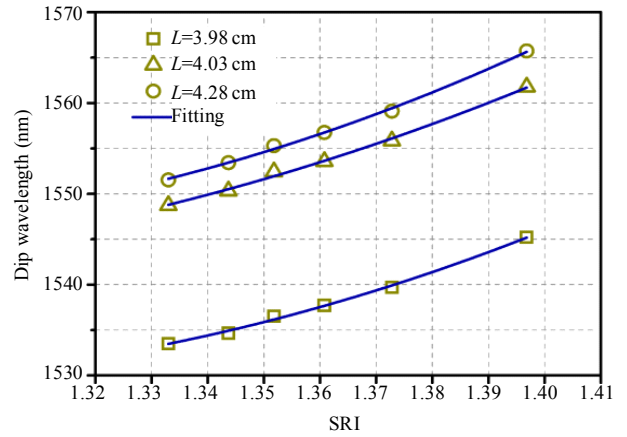
Fig. 6 Dip wavelength shift vs. SRI.
