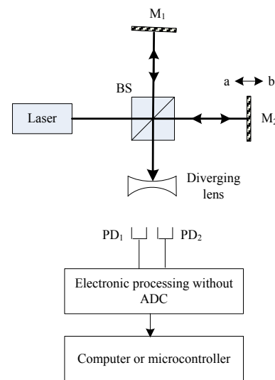
Fig. 1 Block diagram of the displacement sensor.
