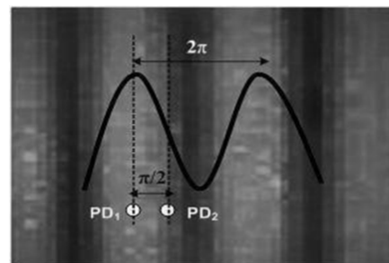
Fig. 2 Fringe pattern.
