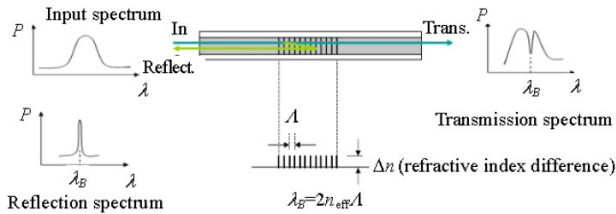
Fig. 1 Functional principle of FBG sensors.
