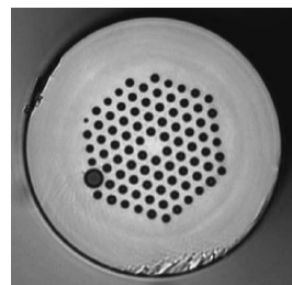
Fig. 27 PCF cross-section of endlessly single mode fiber with inherent asymmetry.
