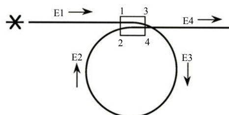
Fig. 1 Schematic of the all fiber ring resonator.
